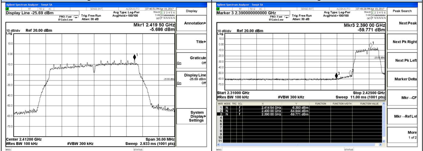
802.11g - Low channel Reference
