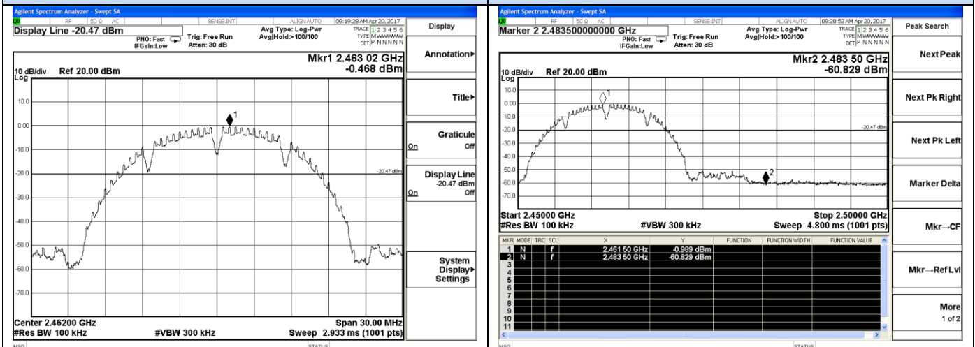
802.11b- High channel Reference
