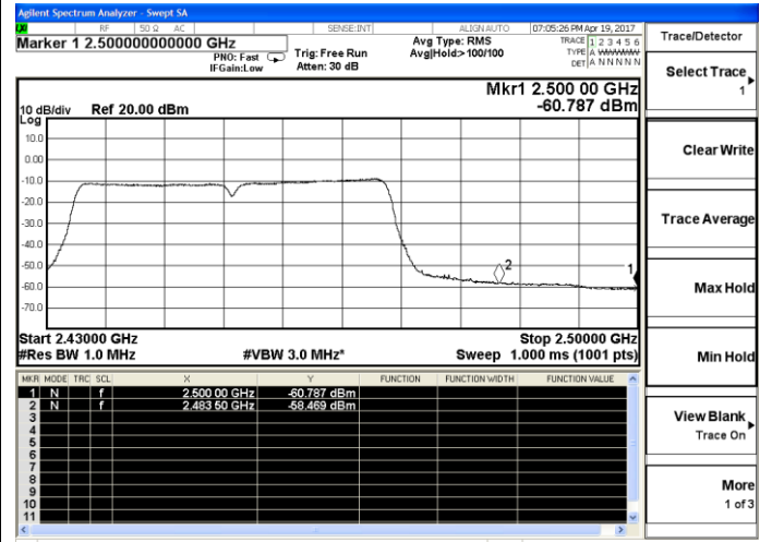
802.11n-HT40 High channel(Average)
