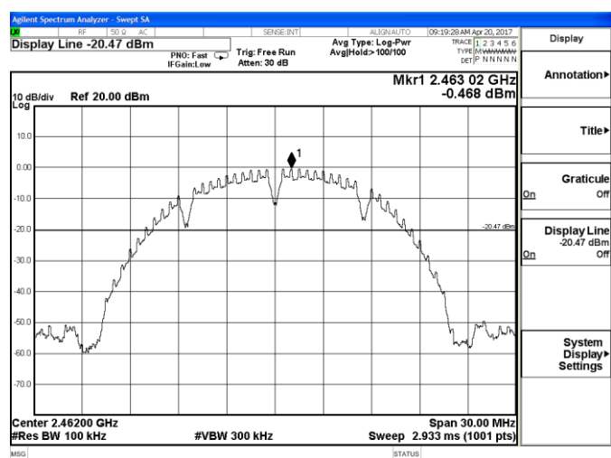
802.11b_High Channel
