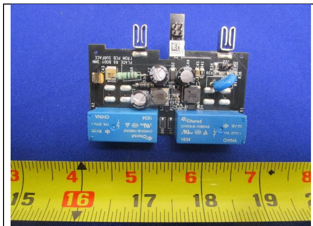
Board Open Bottom View
