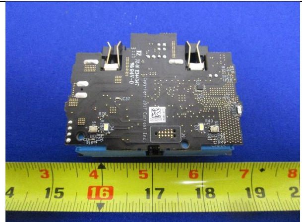
Board - Top View
