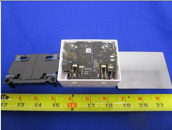
Open Case View - 2
