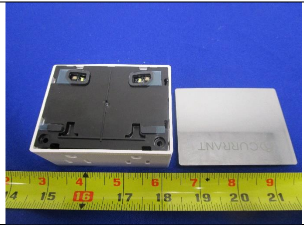
Open Case View - 1
