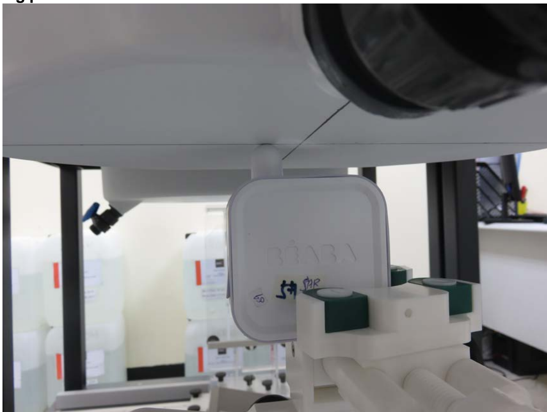
Figure 5 - Top surface with 0mm Separation
