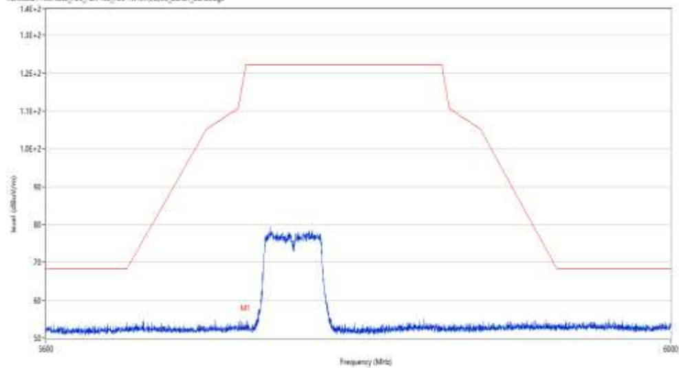
REmission Test case_FCC Part 15E FCC 15.407/55/55_Band4_Bandedge
