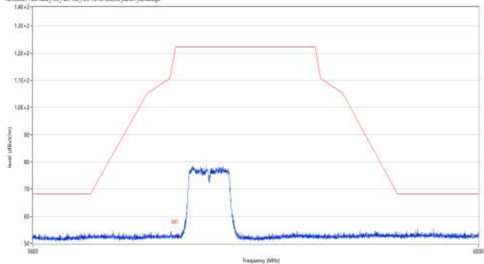
REmission Test case_FCC_Part 15E FCC 15.407(SQ/SS_Band4_Bandedge
