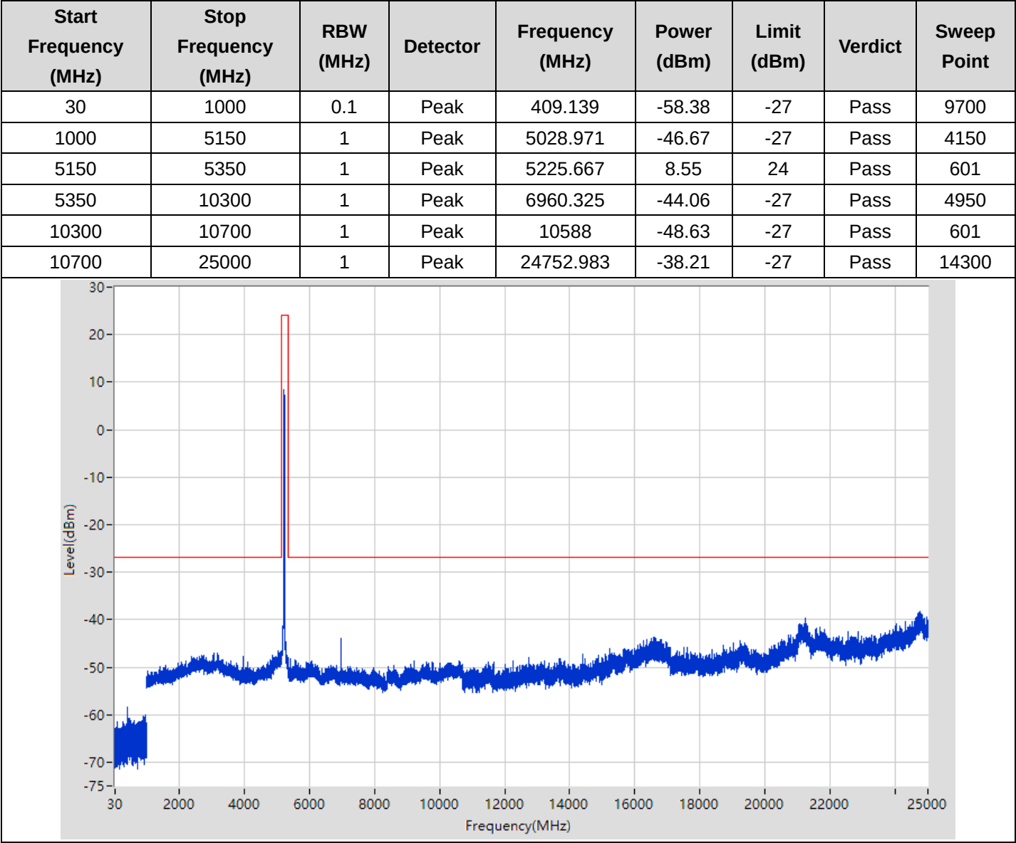
MIMO Undesirable Emission, 30MHz-25GHz, 802.11n(HT20), 5220MHz
