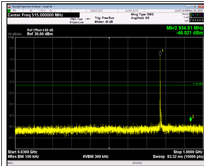
Band13-10MHz-64QAM-23230-1RB#0-Range1:30~1000MHz
