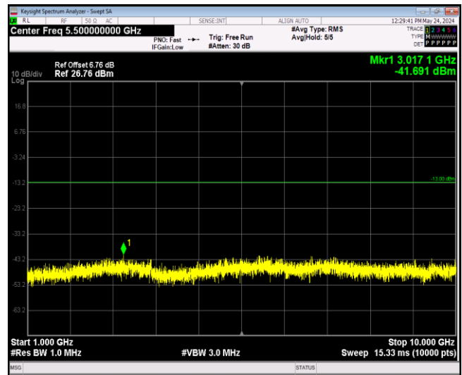
Band13-10MHz-QPSK-23230-1RB#0-Range2:1000~100
