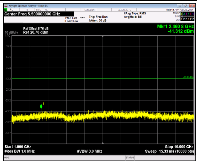
Band12-10MHz-16QAM-23130-1RB#0-Range2:1000~10000MHz
