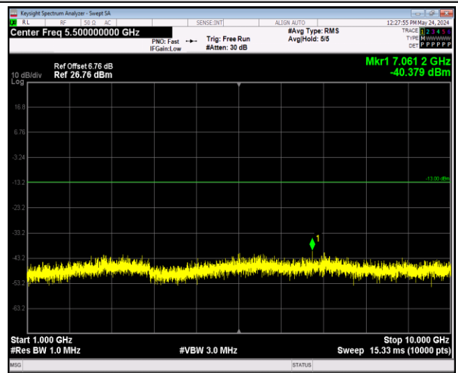
Band13-5MHz-64QAM-23230-1RB#0-Range2:1000~100 00MHz
