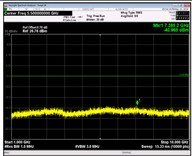
Band12-10MHz-64QAM-23060-1RB#0-Range2:1000~10000MHz
