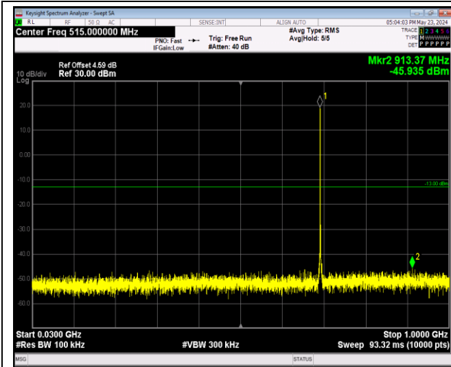
Band12-1.4MHz-16QAM-23095-1RB#0-Range1:30~1000MHz
