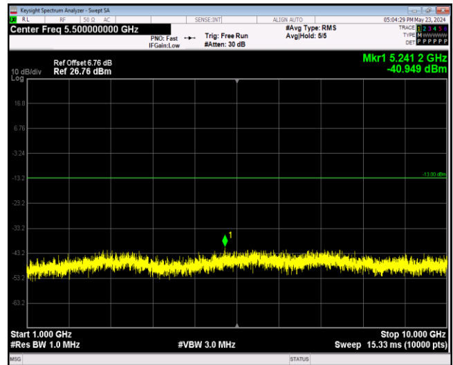
Band12-1.4MHz-64QAM-23095-1RB#0-Range2:1000~10 000MHz
