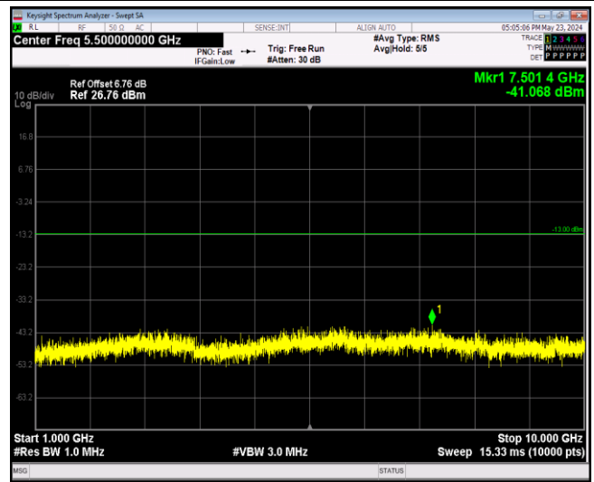
Band12-1.4MHz-16QAM-23173-1RB#0-Range2:1000~10000MHz
