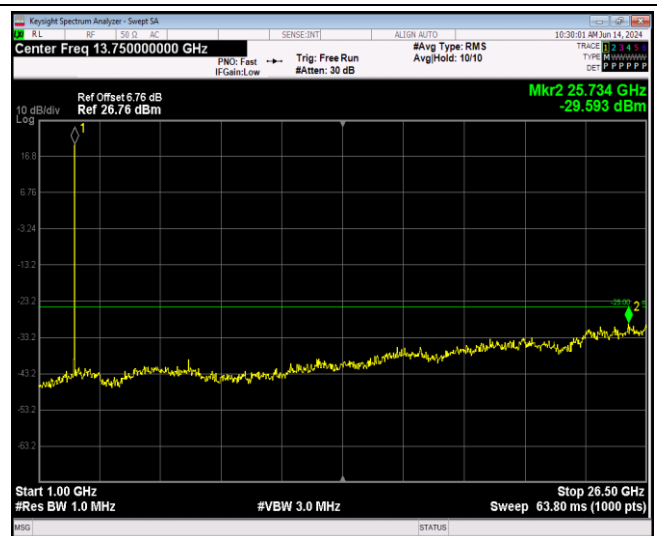
Band41-5MHz-16QAM-40620-1RB#0-Range2:1000~265 00MHz
