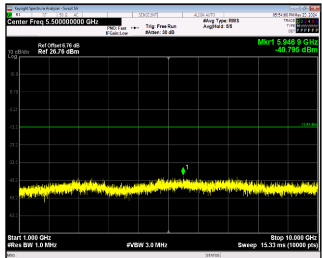
Band12-10MHz-16QAM-23095-1RB#0-Range2:1000~10
