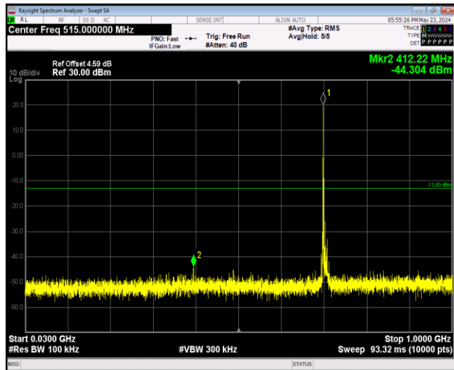
Band12-10MHz-16QAM-23060-1RB#0-Range1:30~10
