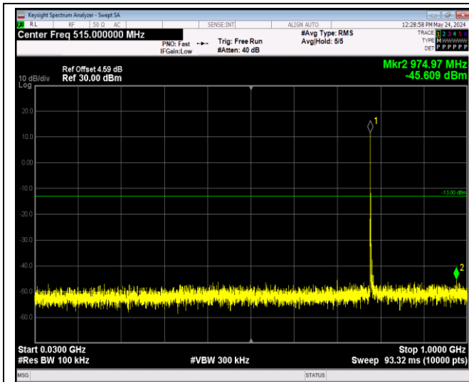
Band13-5MHz-64QAM-23205-1RB#0-Range1:30~100 0MHz
