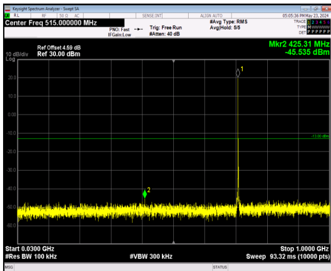
Band12-1.4MHz-16QAM-23017-1RB#0-Range1:30~1 00MHz
