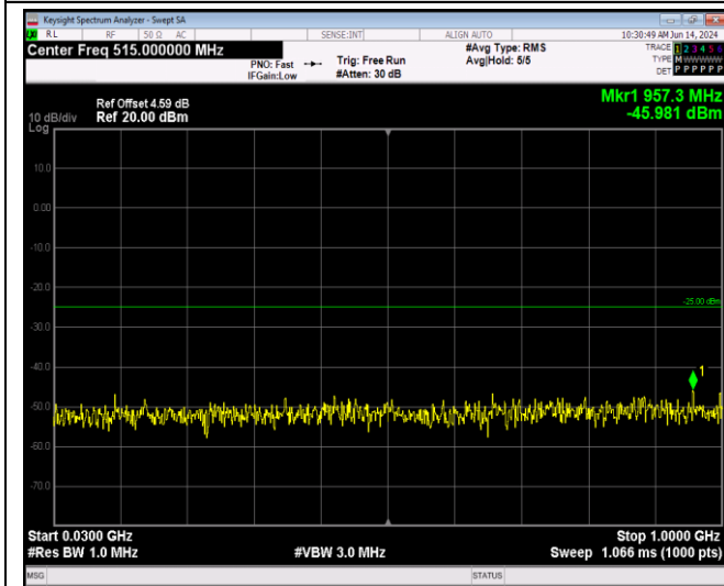
Band41-5MHz-16QAM-41565-1RB#0-Range1:30~100 0MHz
