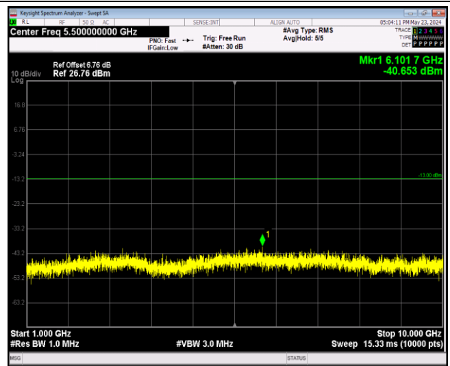
Band12-1.4MHz-16QAM-23095-1RB#0-Range2:1000~10000MHz
