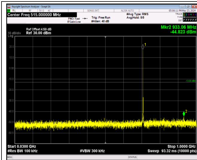
Band12-10MHz-QPSK-23060-1RB#0-Range1:30~100 0MHz
