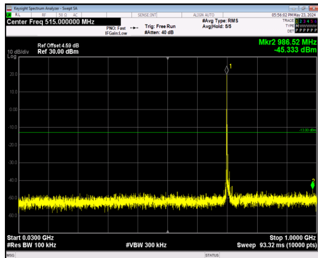
Band13-5MHz-QPSK-23205-1RB#0-Range1:30~1000
