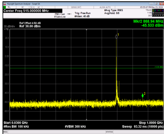
Band12-10MHz-64QAM-23130-1RB#0-Range1:30~10
