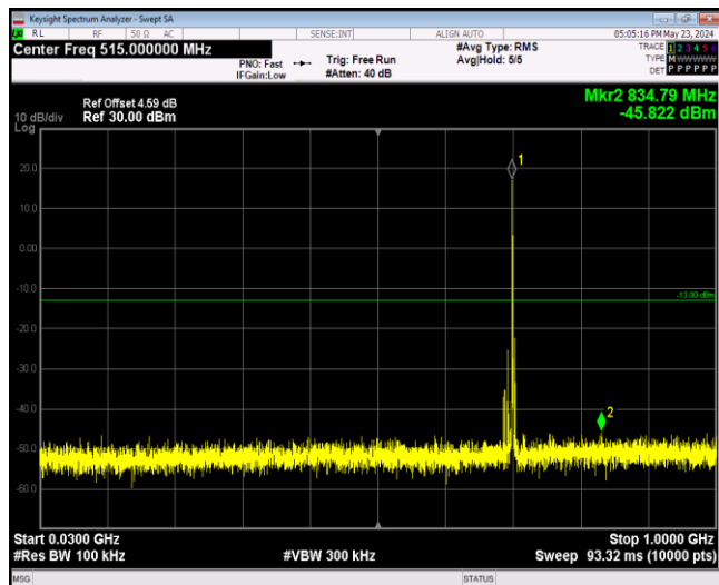
Band12-1.4MHz-64QAM-23173-1RB#0-Range1:30~1 000MHz
