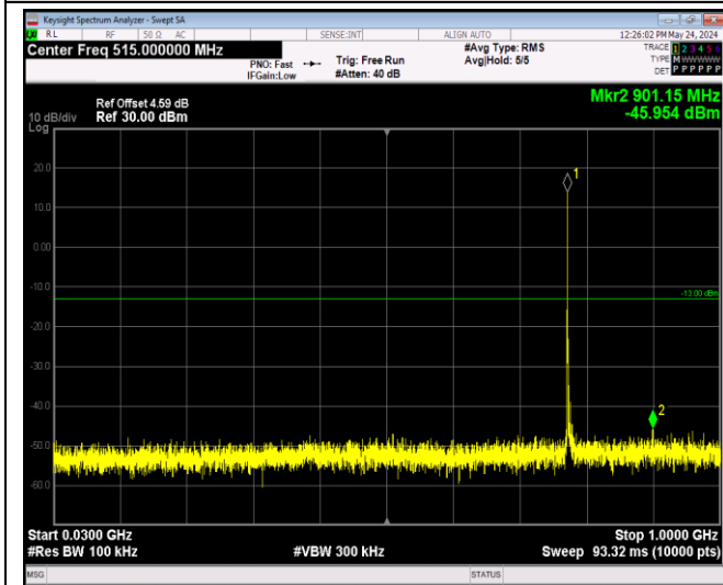
Band13-5MHz-64QAM-23230-1RB#0-Range1:30~100 0MHz
