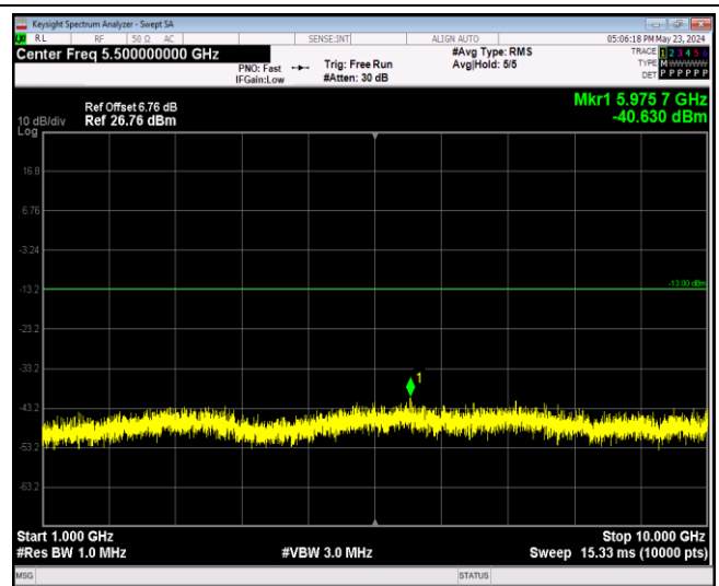
Band12-10MHz-QPSK-23060-1RB#0-Range2:1000~100 00MHz
