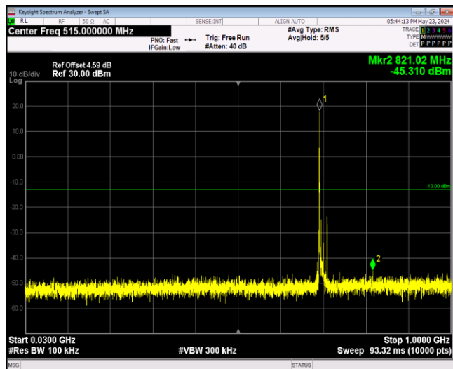
Band12-10MHz-16QAM-23095-1RB#0-Range1:30~10
