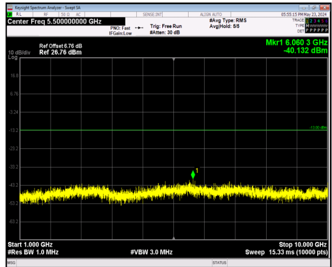
Band12-10MHz-64QAM-23130-1RB#0-Range2:1000~10
