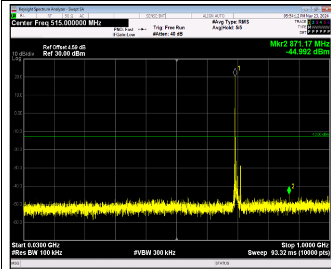
Band12-10MHz-64QAM-23060-1RB#0-Range1:30~1000MHz
