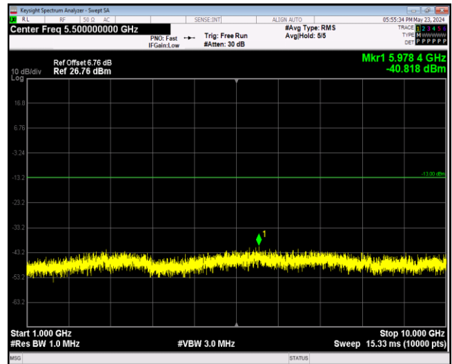
Band12-10MHz-16QAM-23060-1RB#0-Range2:1000~10
