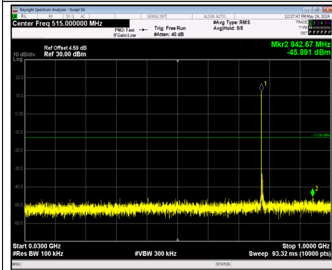
Band13-5MHz-64QAM-23230-1RB#0-Range1:30~100 0MHz
