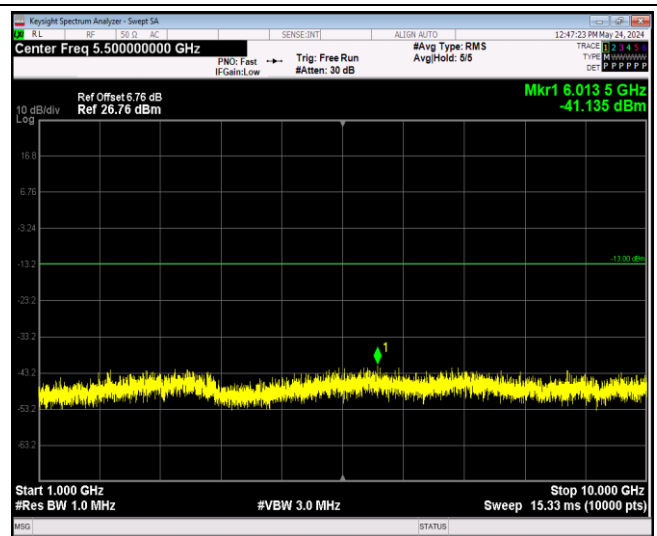
Band13-10MHz-64QAM-23230-1RB#0-Range2:1000~10000MHz
