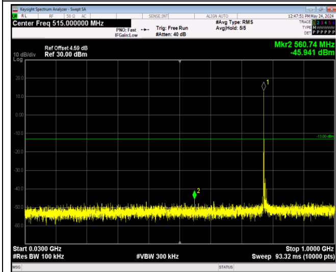
Band41-5MHz-QPSK-39675-1RB#0-Range1:30~1000MHz
