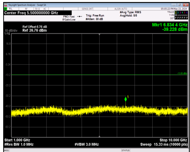
Band12-1.4MHz-64QAM-23173-1RB#0-Range2:1000~10 000MHz
