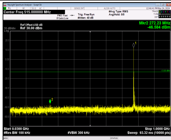
Band13-10MHz-16QAM-23230-1RB#0-Range1:30~10
