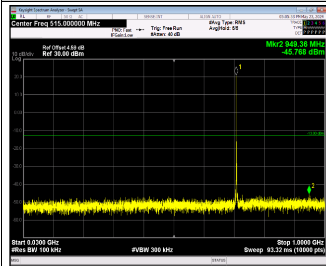
Band12-1.4MHz-16QAM-23173-1RB#0-Range1:30~1000MHz
