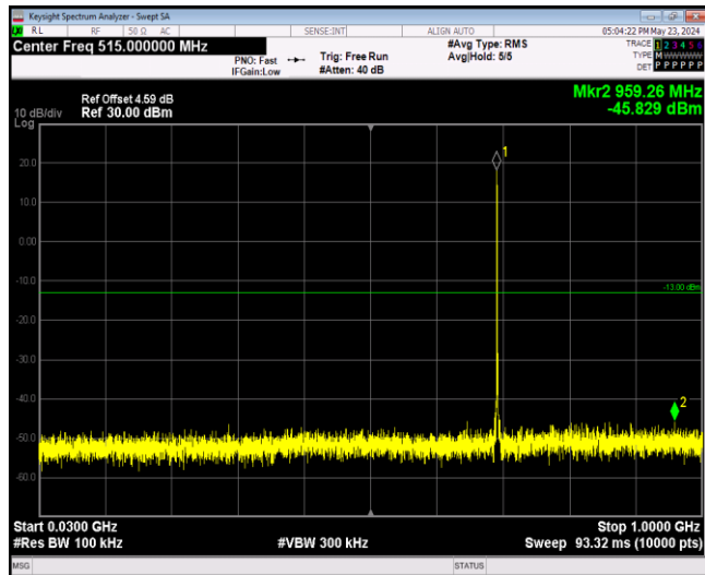
Band12-1.4MHz-64QAM-23095-1RB#0-Range1:30~1 000MHz
