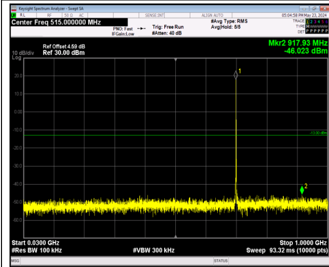
Band12-1.4MHz-16QAM-23173-1RB#0-Range1:30~1000MHz
