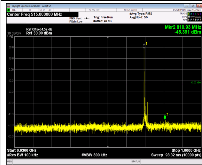
Band12-10MHz-16QAM-23130-1RB#0-Range1:30~1000MHz
