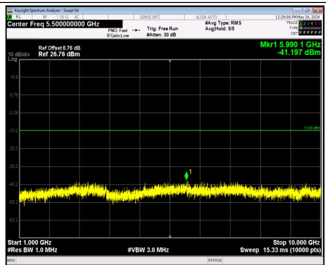
Band13-5MHz-64QAM-23205-1RB#0-Range2:1000~100 00MHz
