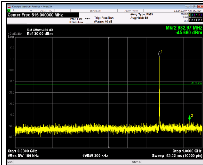
Band13-5MHz-QPSK-23230-1RB#0-Range1:30~1000 MHz
