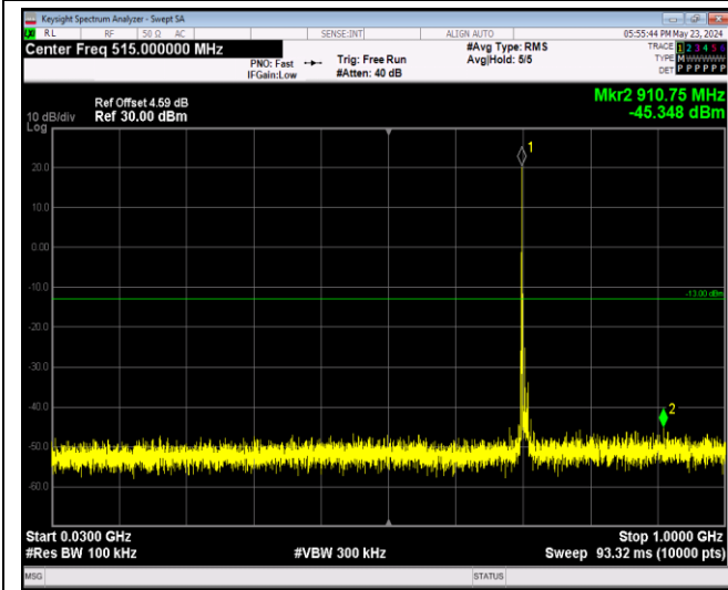
Band12-10MHz-64QAM-23060-1RB#0-Range1:30~1000MHz
