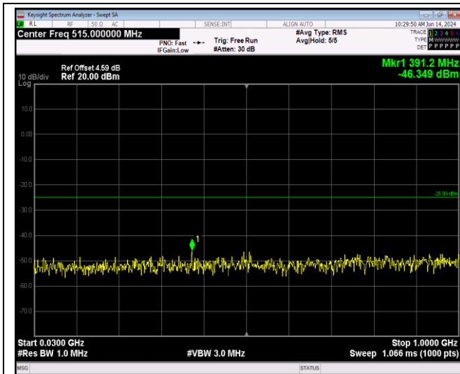
Band41-5MHz-16QAM-40620-1RB#0-Range1:30~100 0MHz
