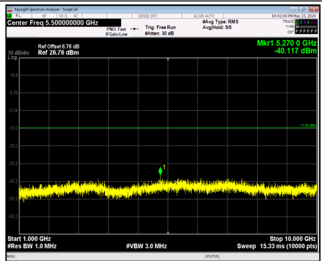
Band5-10MHz-64QAM-20450-1RB#0-Range2:1000~100 00MHz
