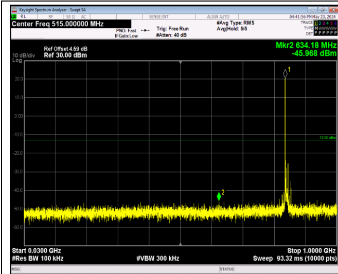
Band5-10MHz-64QAM-20450-1RB#0-Range1:30~100 0MHz
