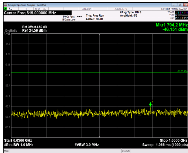
Band2-20MHz-64QAM-19100-1RB#0-Range1:30~100 0MHz
