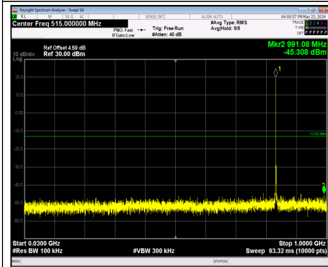
Band5-1.4MHz-QPSK-20525-1RB#0-Range1:30~100 OMHz
