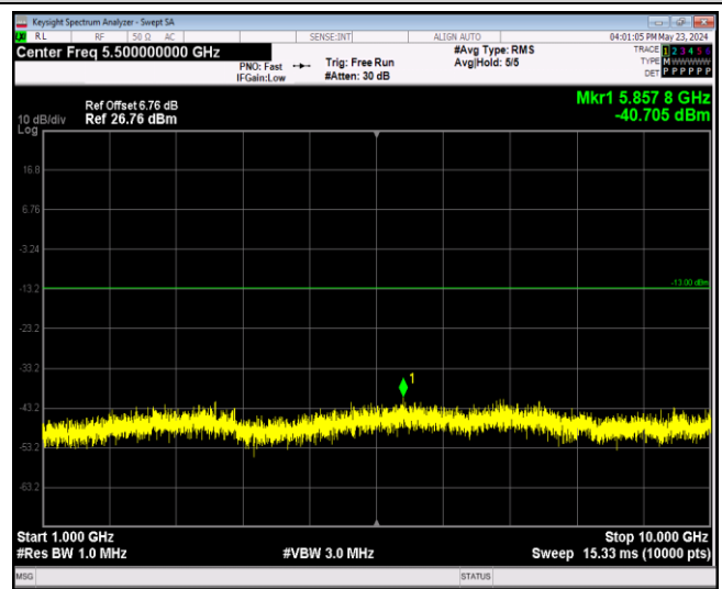
Band5-1.4MHz-QPSK-20525-1RB#0-Range2:1000~1000 OMHz
