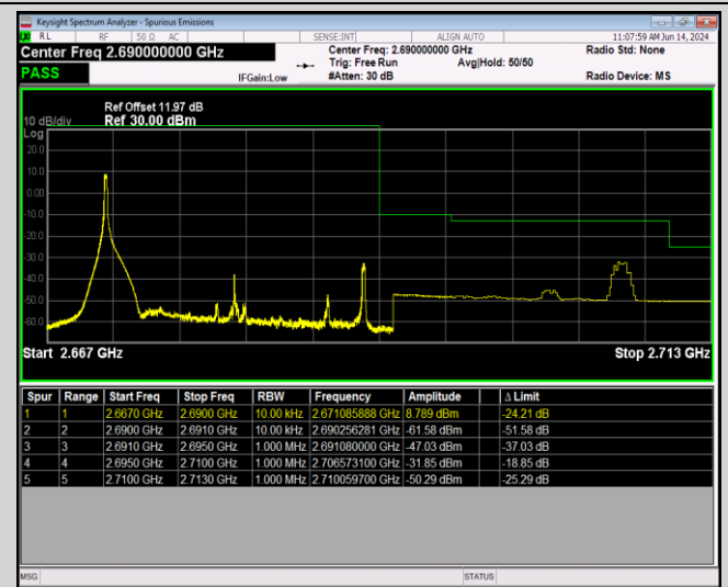
Band41-20MHz-QPSK-41490-100RB#0
