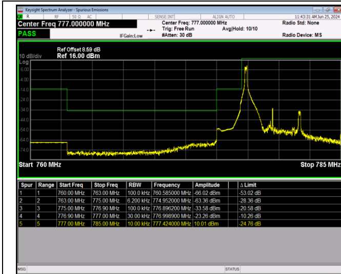
Band13-5MHz-64QAM-23205-25RB#0
