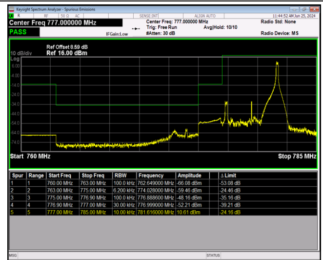
Band13-5MHz-16QAM-23255-1RB#0
