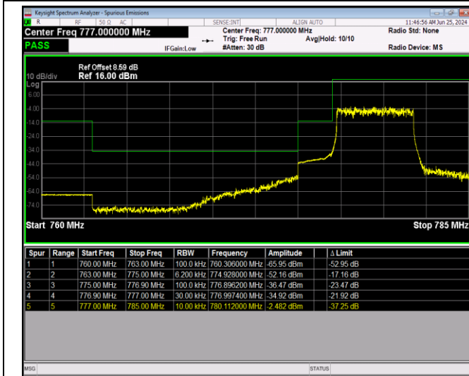
Band13-5MHz-16QAM-23255-1RB#24
