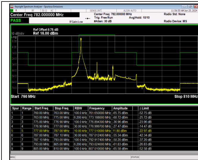
Band13-10MHz-QPSK-23230-50RB#0
