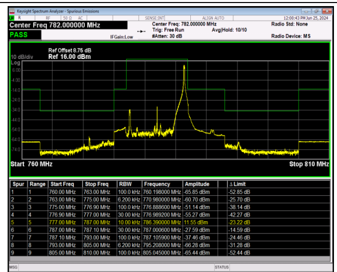
Band13-10MHz-16QAM-23230-1RB#0
