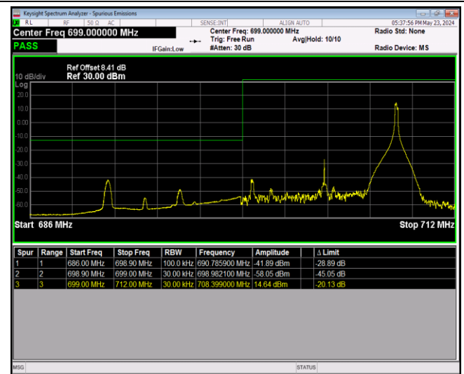
Band12-10MHz-64QAM-23130-1RB#0
