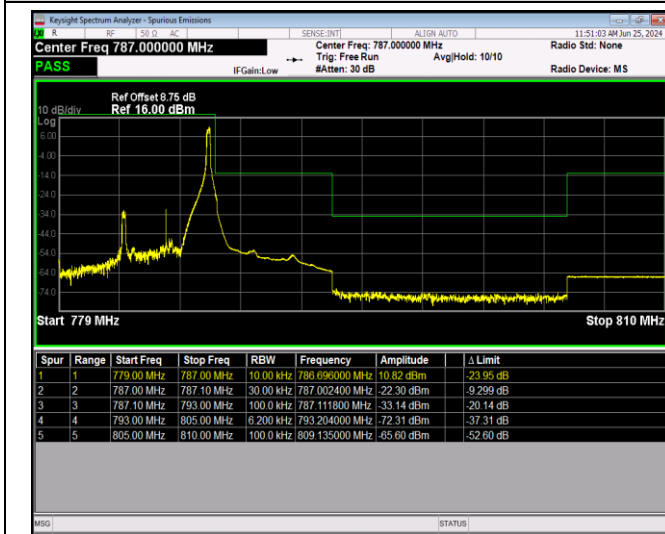
Band13-5MHz-64QAM-23205-1RB#0
