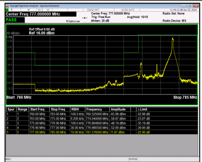
Band13-5MHz-QPSK-23255-1RB#0
