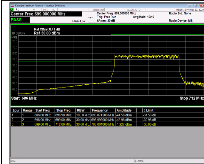
Band12-10MHz-64QAM-23130-1RB#49
