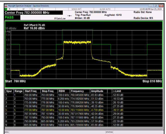
Band13-10MHz-64QAM-23230-1RB#49
