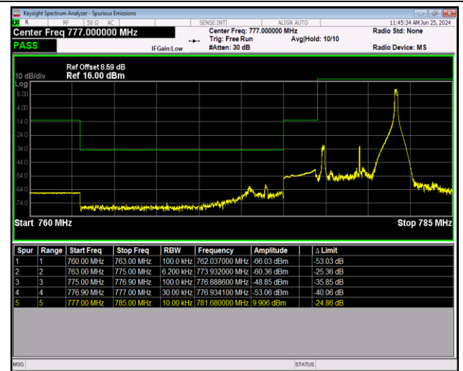
Band13-5MHz-64QAM-23255-1RB#0
