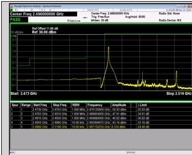
Band41-20MHz-QPSK-39750-100RB#0
