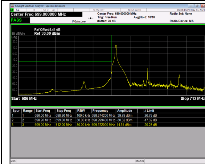
Band12-10MHz-16QAM-23060-50RB#0
