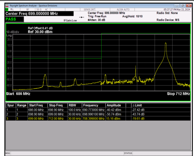
Band12-10MHz-16QAM-23130-1RB#0
