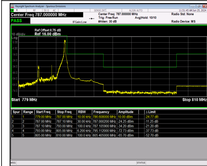
Band13-10MHz-QPSK-23230-1RB#0
