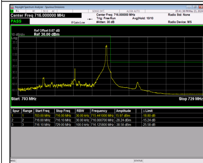
Band12-10MHz-64QAM-23060-1RB#0
