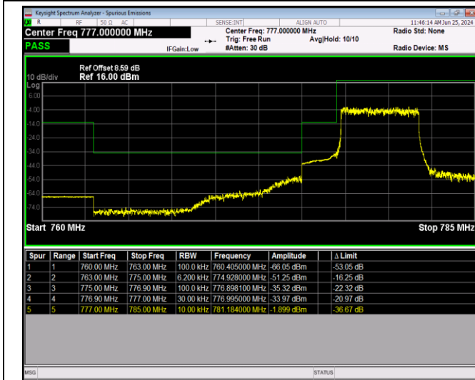
Band13-5MHz-QPSK-23255-1RB#24
