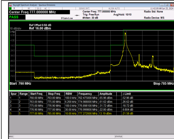
Band13-5MHz-QPSK-23205-25RB#0
