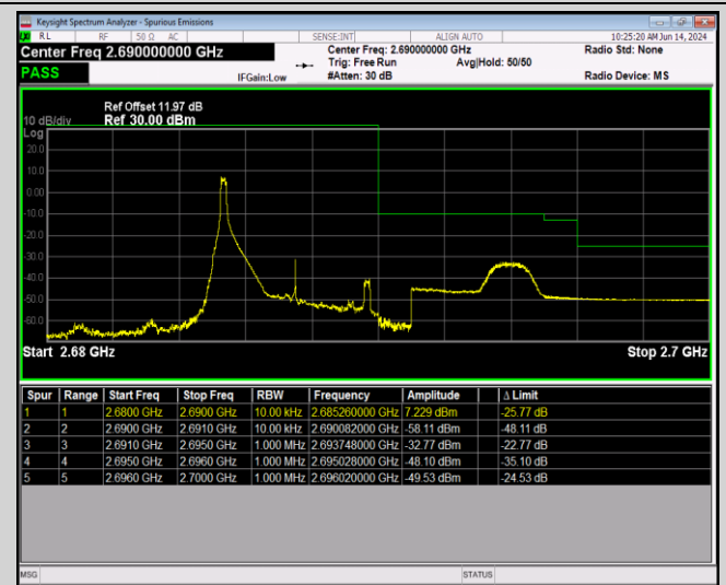
Band41-5MHz-16QAM-41565-25RB#0
