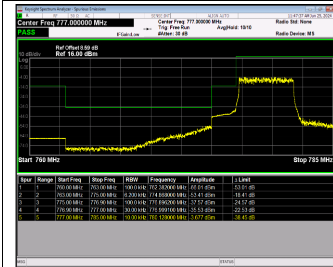
Band13-5MHz-64QAM-23255-1RB#24
