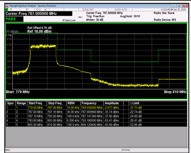
Band13-10MHz-QPSK-23230-1RB#49
