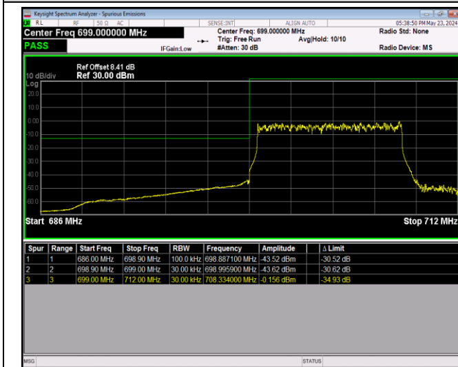
Band12-10MHz-16QAM-23130-1RB#49
