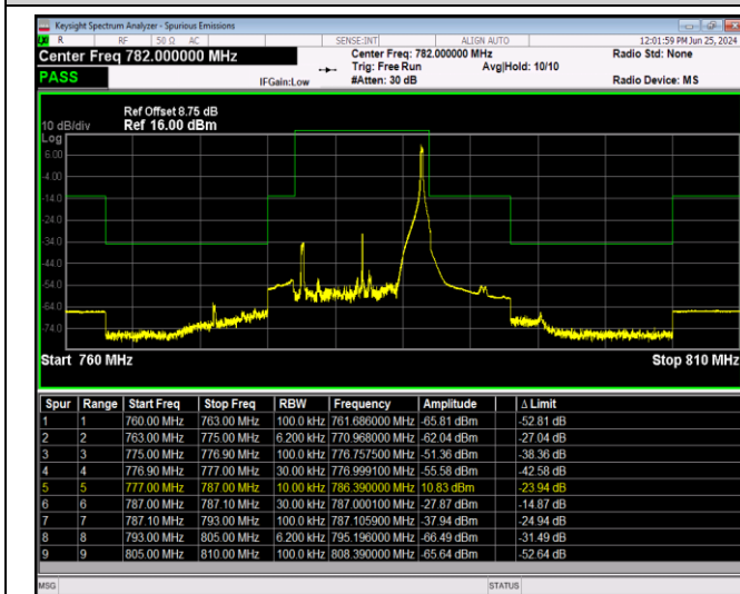
Band13-10MHz-64QAM-23230-1RB#0
