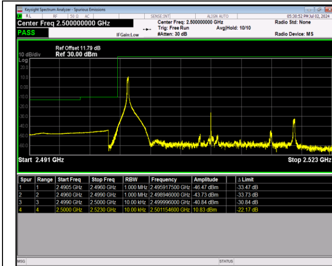
Band7-20MHz-16QAM-20850-100RB#0
