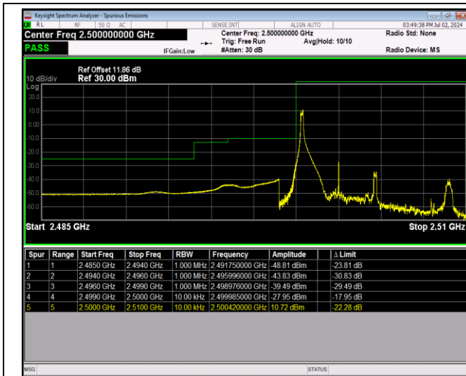
Band7-5MHz-16QAM-20775-25RB#0
