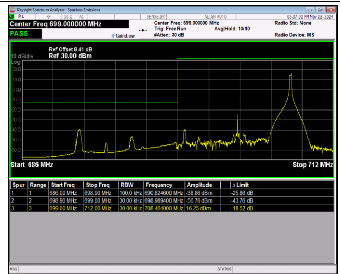
Band12-10MHz-QPSK-23130-1RB#0
