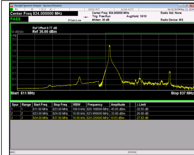
Band5-10MHz-16QAM-20450-50RB#0
