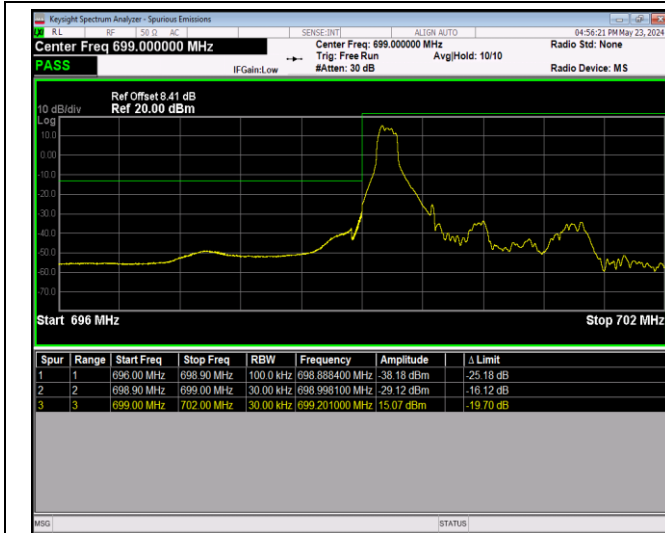
Band12-1.4MHz-64QAM-23017-6RB#0
