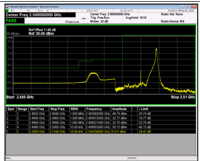
Band7-5MHz-64QAM-21425-1RB#0
