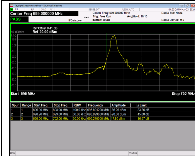
Band12-1.4MHz-QPSK-23017-6RB#0
