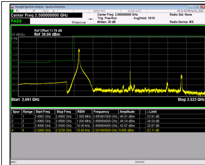
Band7-20MHz-64QAM-20850-100RB#0
