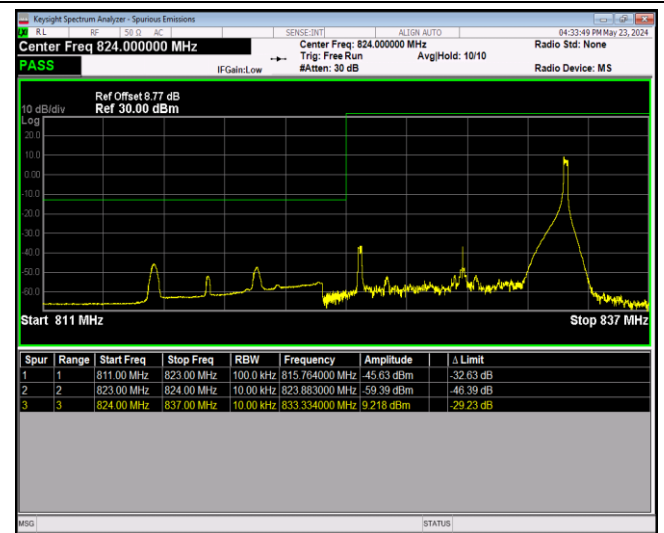
Band5-10MHz-64QAM-20600-1RB#0
