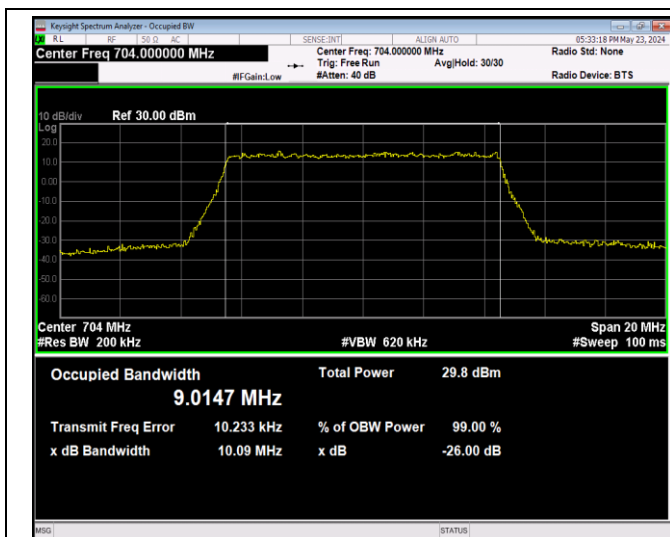
Band12-10MHz-16QAM-23130-50RB#0
