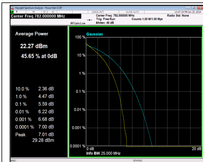
Band13-10MHz-64QAM-23230-50RB#0
