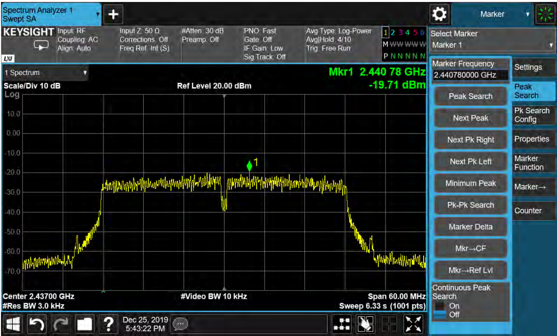
Figure 47: Power Spectral Density, 802.11n(HT40), 2437MHz
