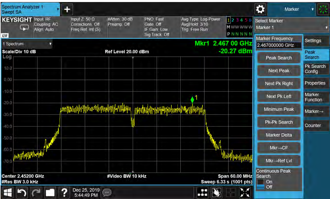
Figure 48: Power Spectral Density, 802.11n(HT40), 2452MHz
