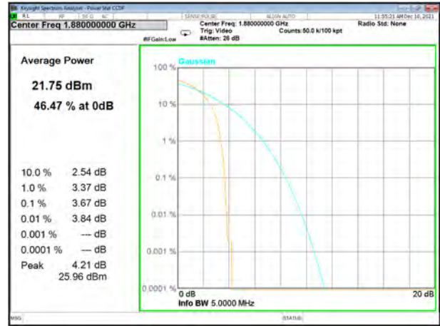
HSPA Band 2_Middle
