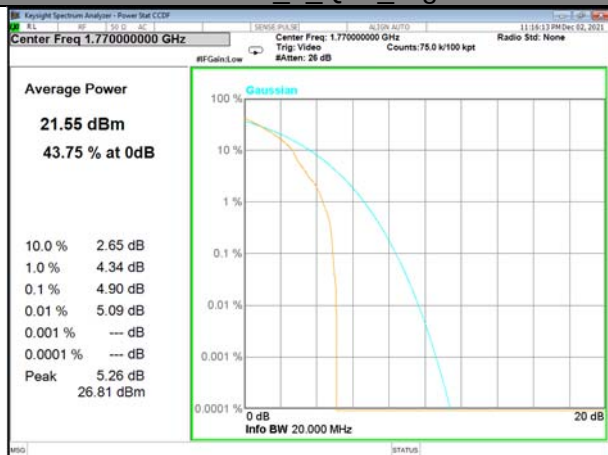
Band 66_1_Q16_High
