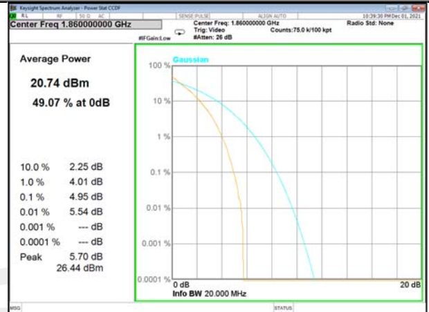
Band 2_100_Q16_Low
