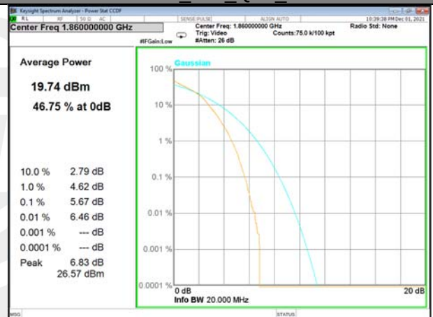
Band 2_100_QPSK_Middle
