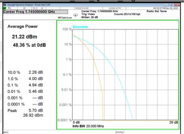
Band 4_100_Q16_High
