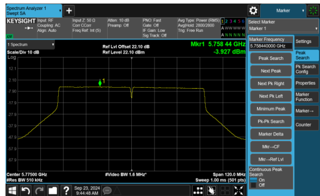
Channel 155 (5775MHz)
