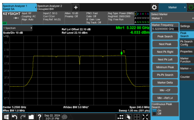
Channel 50 (5250MHz)
