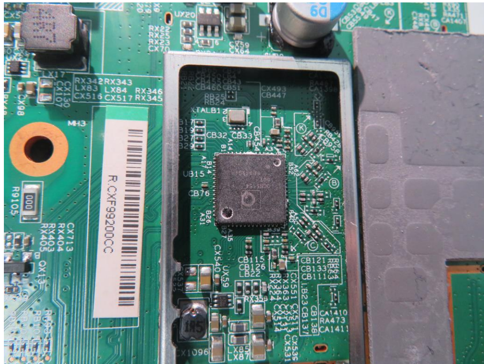
(13) EUT Photo_AP321e
