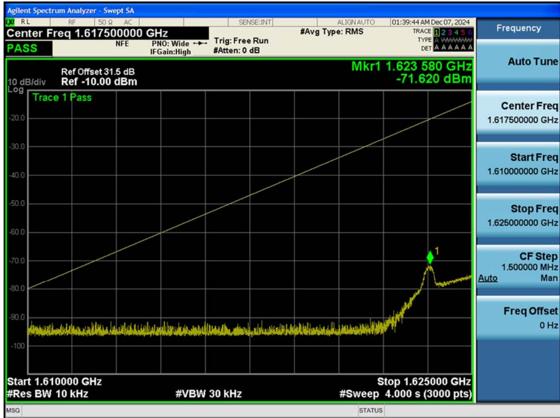
LTE24_5 M_ Ligado_Discrete emissions_1610-1625 MHz_Low_QPSK_1RB
