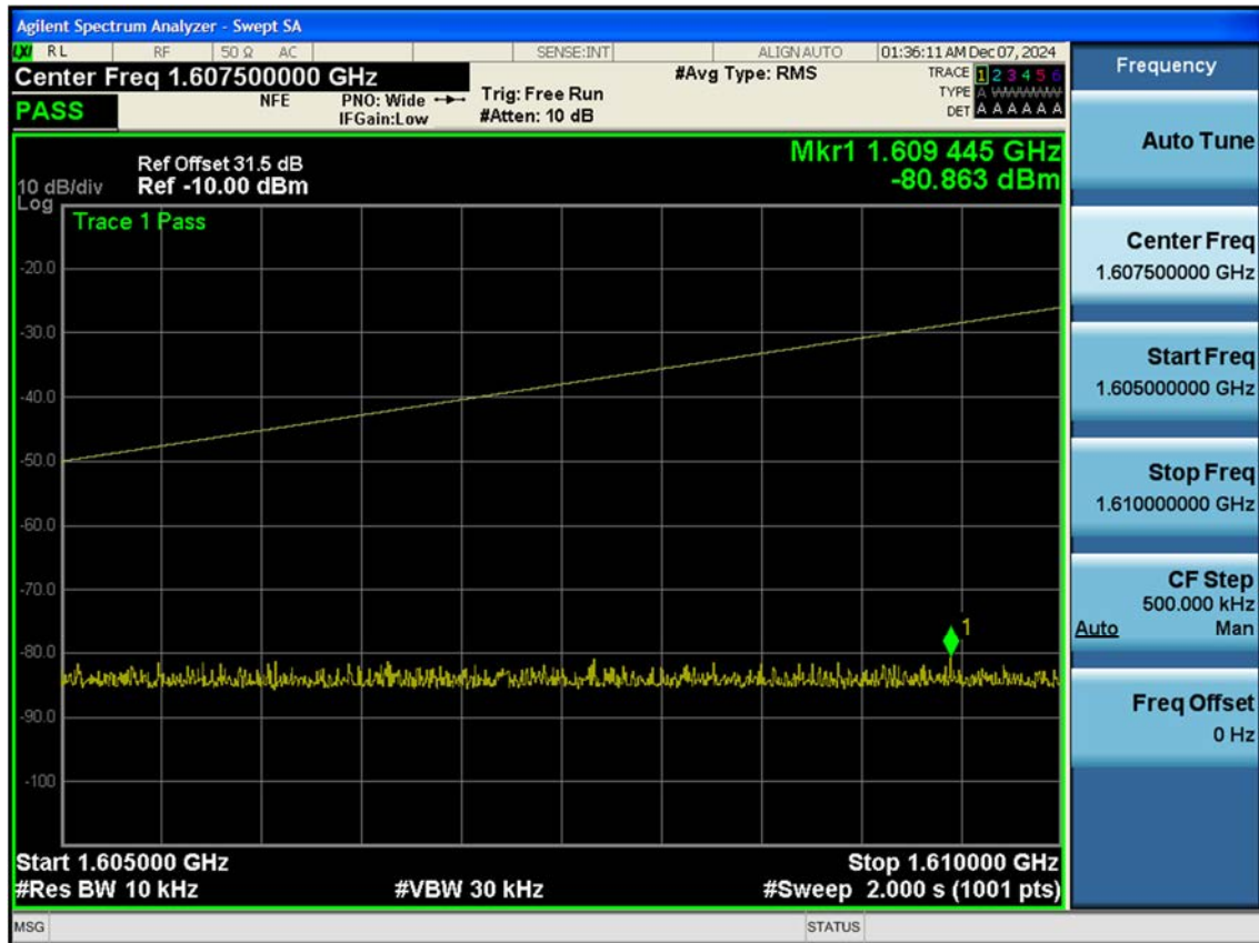
LTE24_5 M_Protection_Narrow(2)_Low_QPSK_1RB
