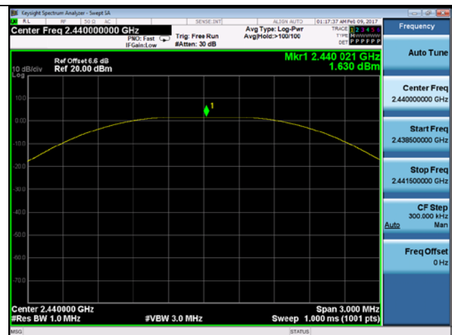
Output Power –Bluetooth LE 2440MHz
