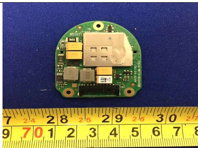
Internal PCBA 1 with Shielding Top View
