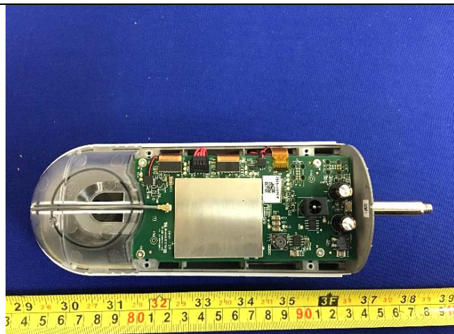
EUT: Cover Off Rear View
