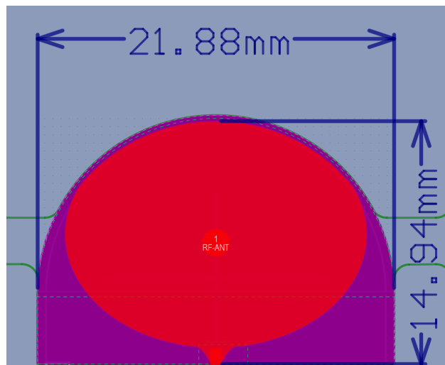
Figure 1: Antenna Dimensions
