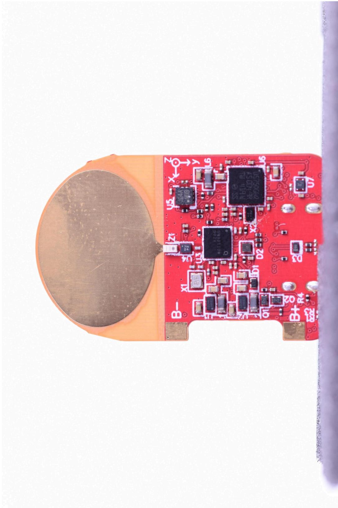
PT301 Internal Board Front View - Zoom / No Ruler
