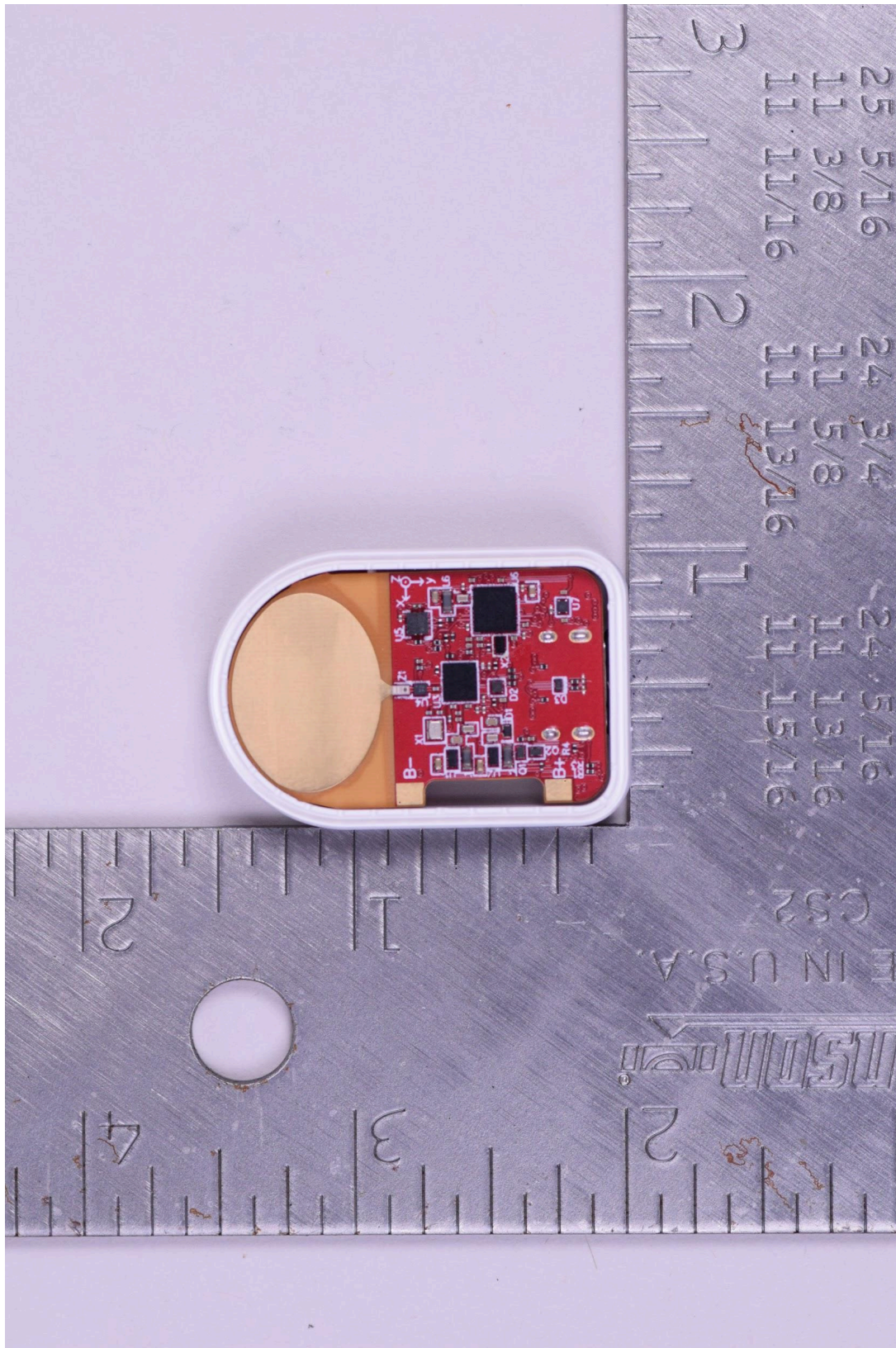
PT301 Internal Board In Open Enclosure w/o battery
