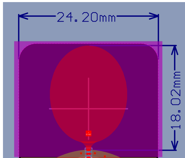
Figure 1: Antenna Dimensions
