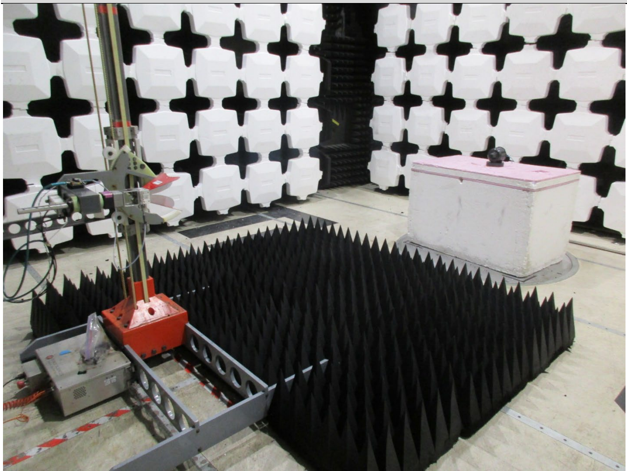
Radiated Testing, Above 1 GHz #1
