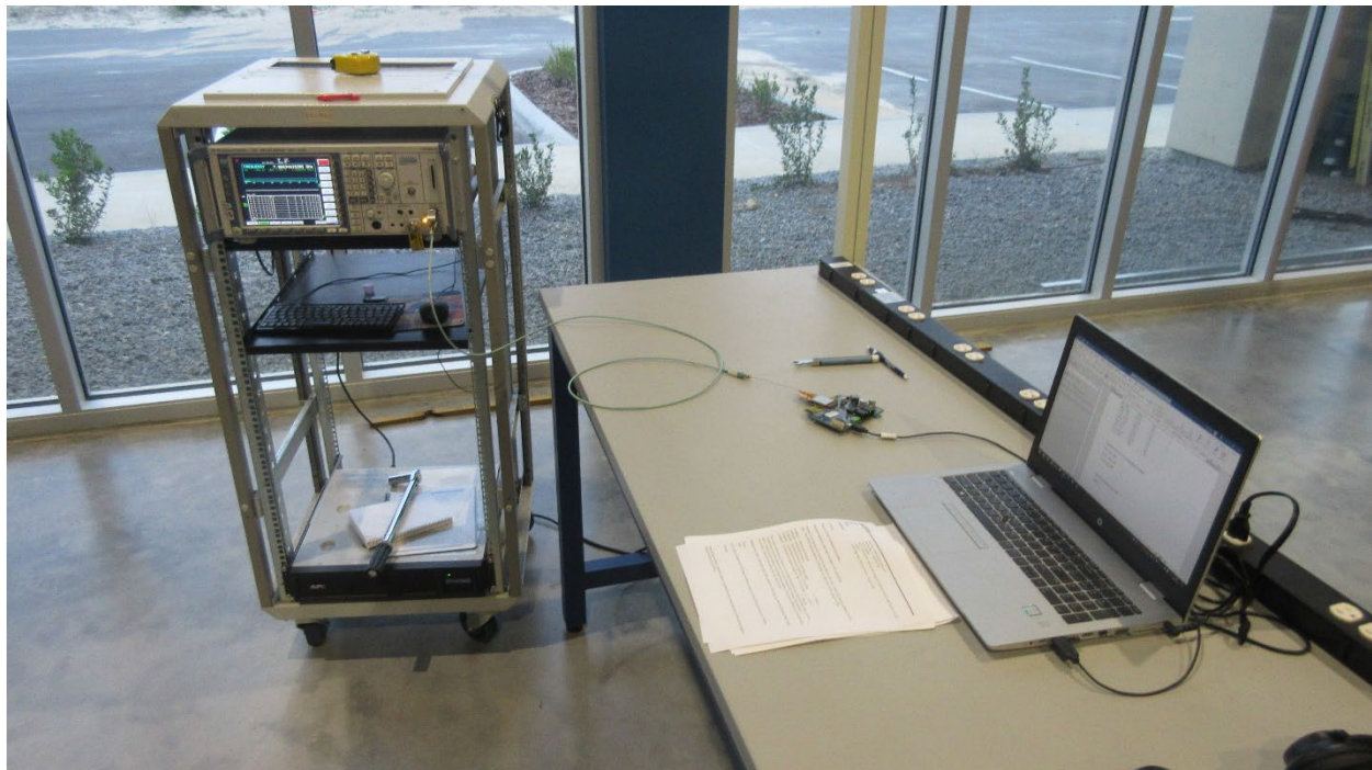
Conducted Test Setup, #1
