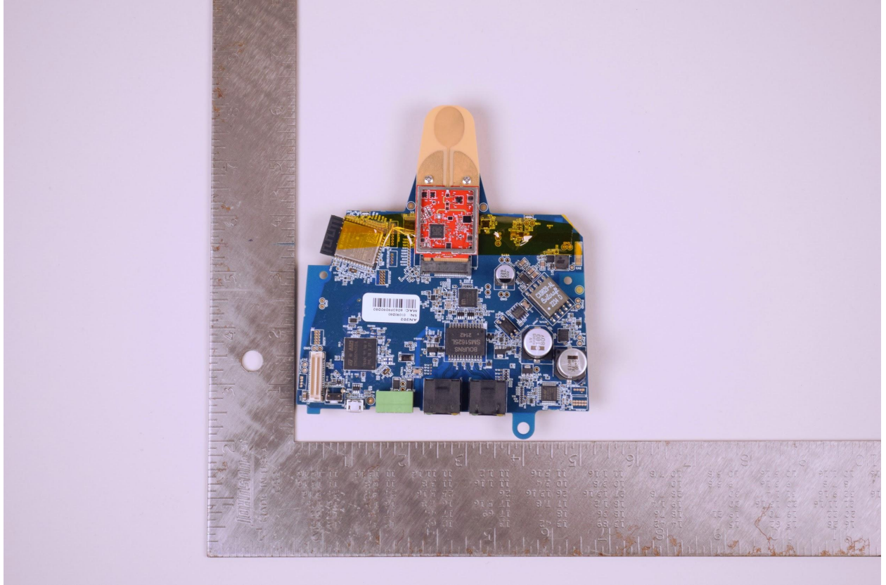
AN203 Internal Board Front View without Shield
