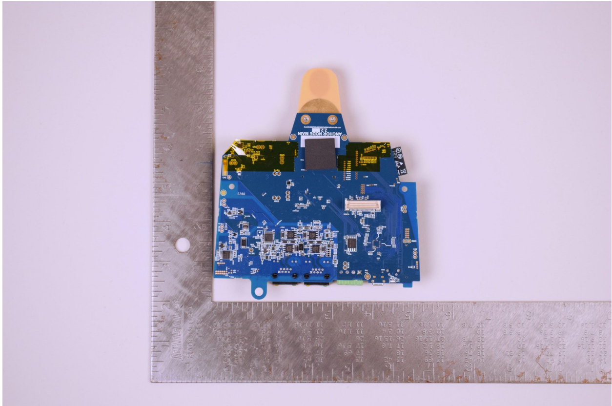
AN203 Internal Board Back View
