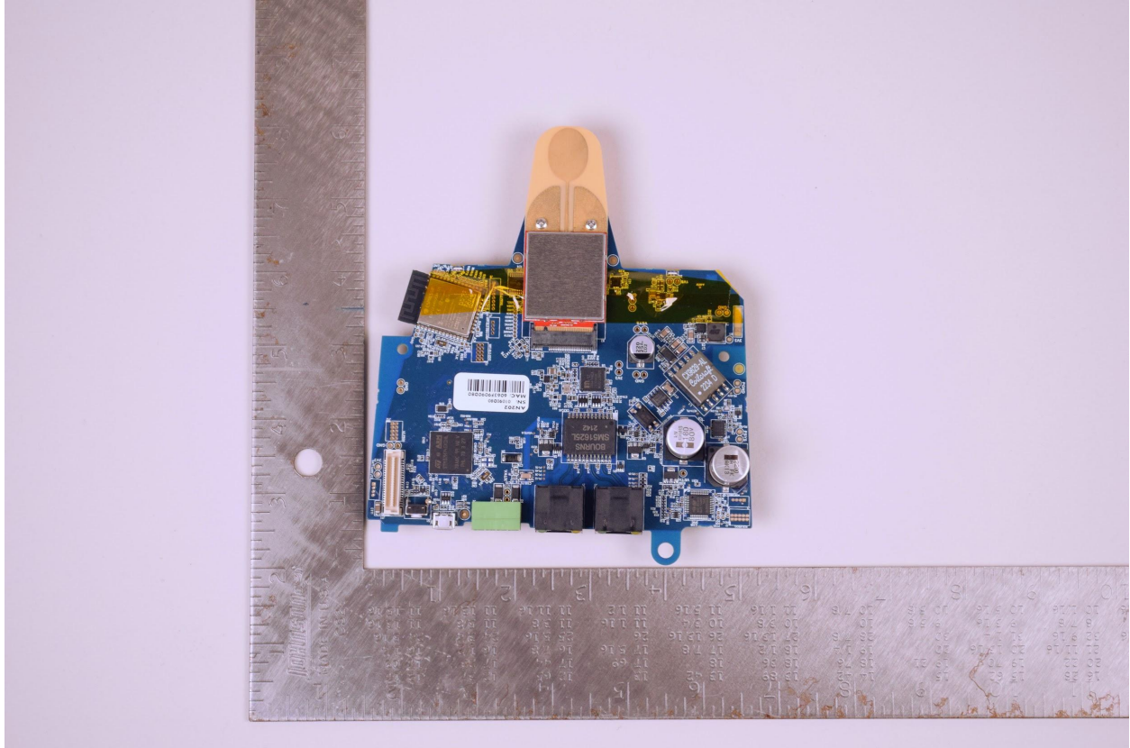
AN203 Internal Board Front View with Shield
