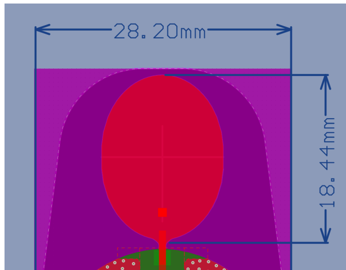
Figure 1: Antenna Dimensions
