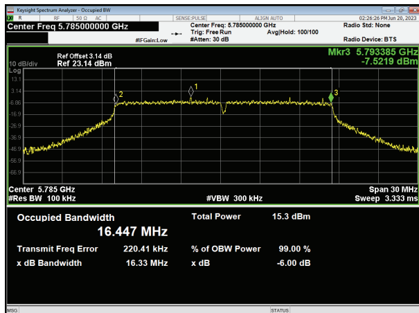
(802.11a20) 6dB Bandwidth plot on channel 157
