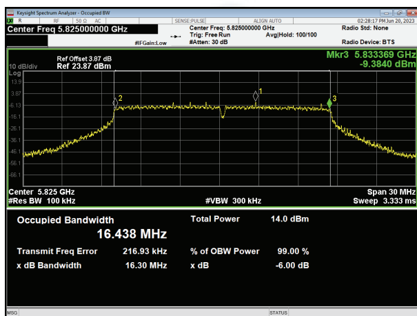
(802.11a20) 6dB Bandwidth plot on channel 165
