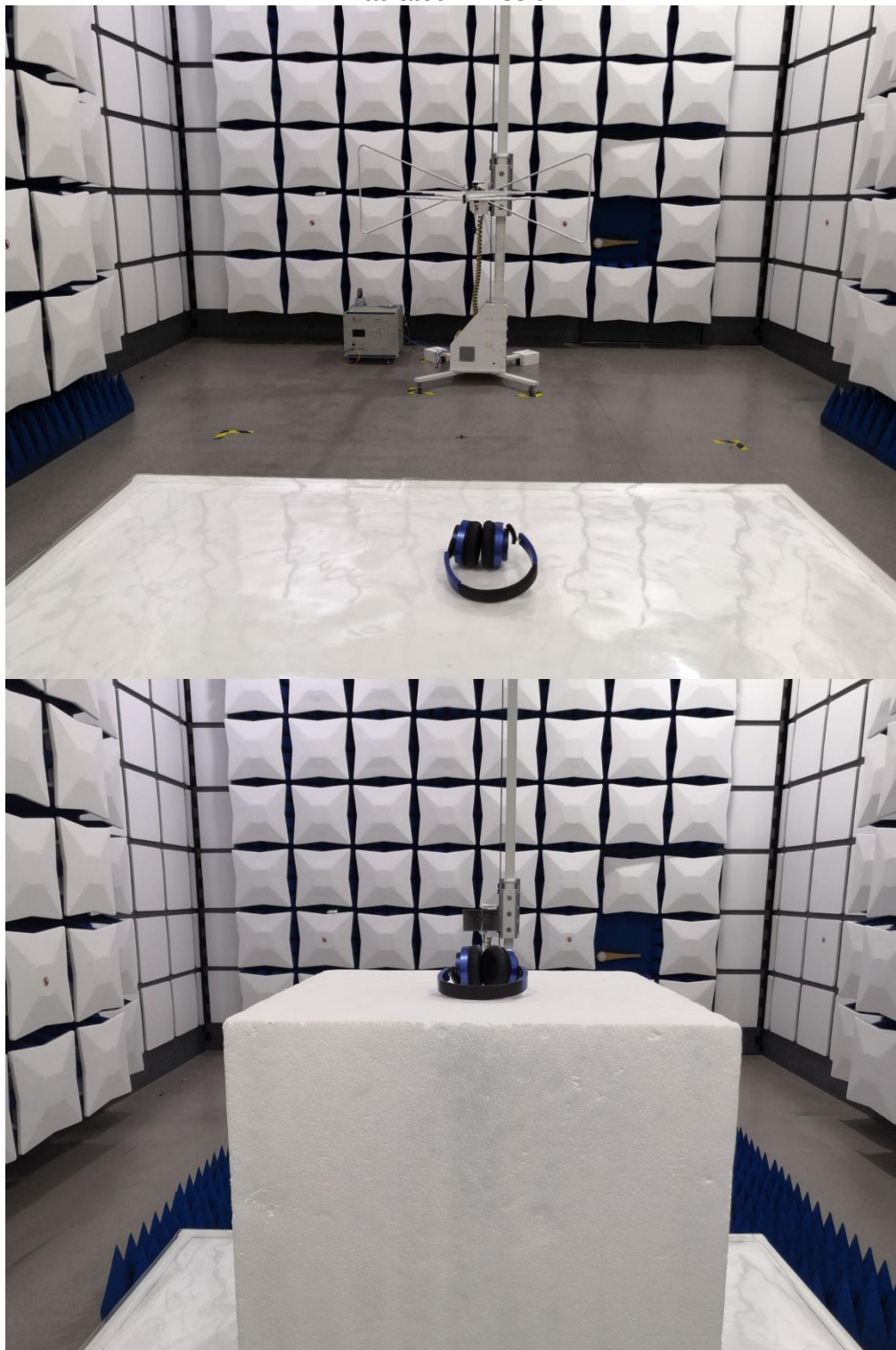
Radiated Emission
