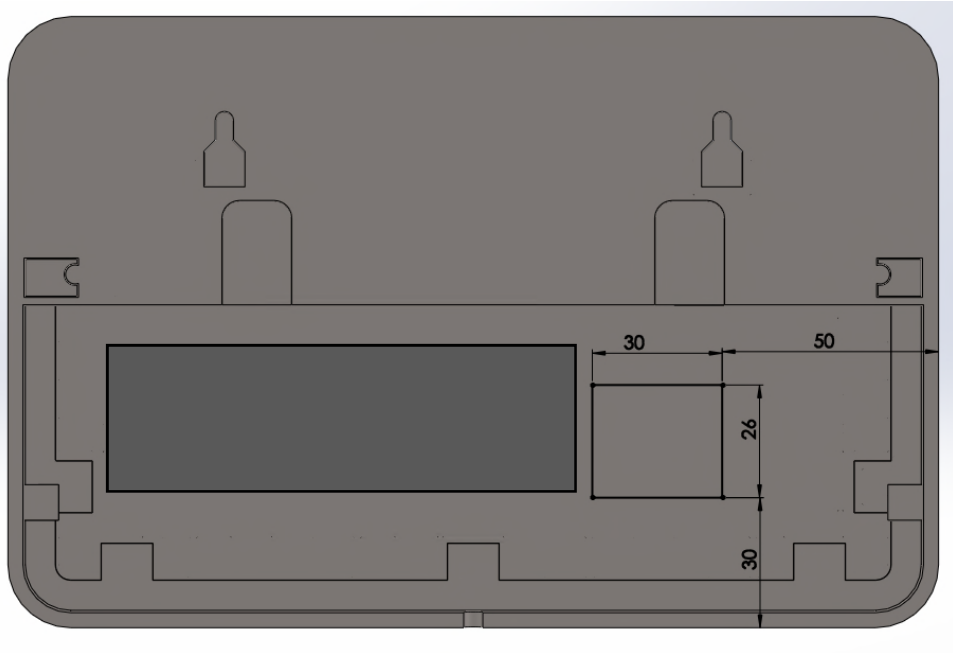
Figure 3- Back face of Action Cam User device showing positioning of labels.
