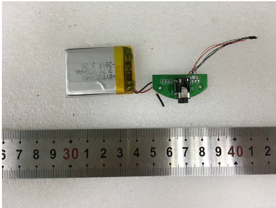
EUT – Power Board Front View
