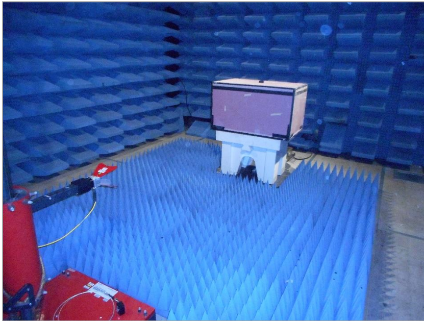
Figure 4: Radiated Emissions (frequency range: 1GHz \leftrightarrow 18GHz) Test Setup
