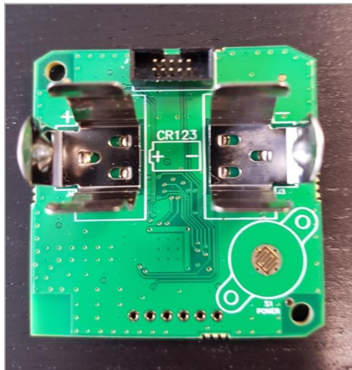
PCB TOP (no battery)
