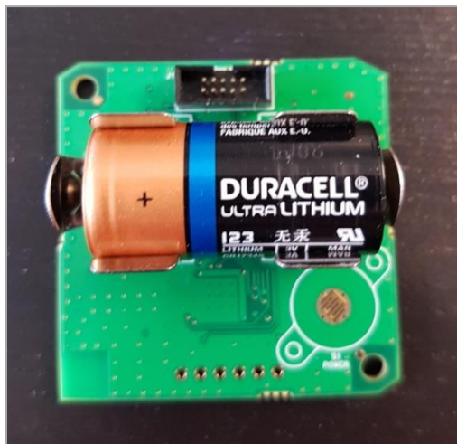
PCB TOP (with battery)
