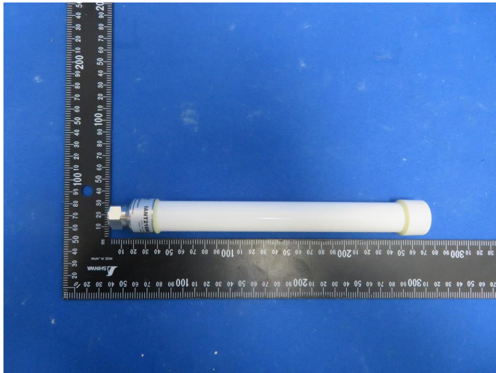
(7) EUT Photo (Omni Antenna)
