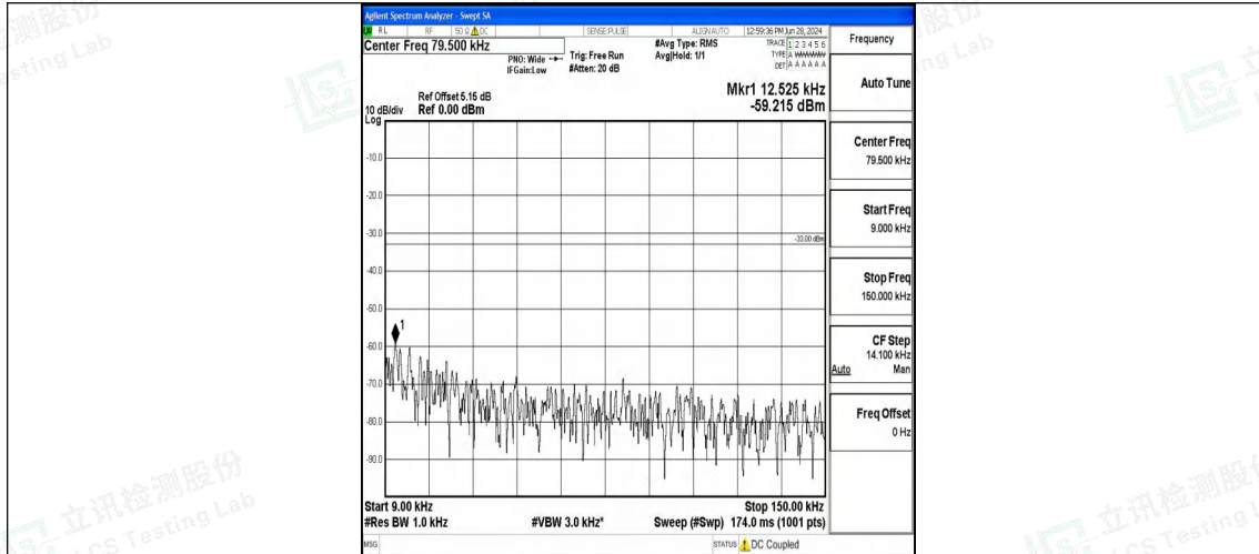
Band12_10MHz_QPSK_23130_1RB#0_0.009~0.15_0.009~0.15
