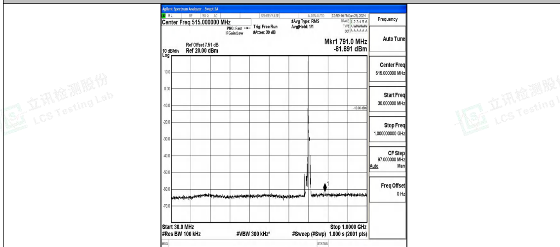
Band12_10MHz_QPSK_23130_1RB#0_30~1000_30~1000
