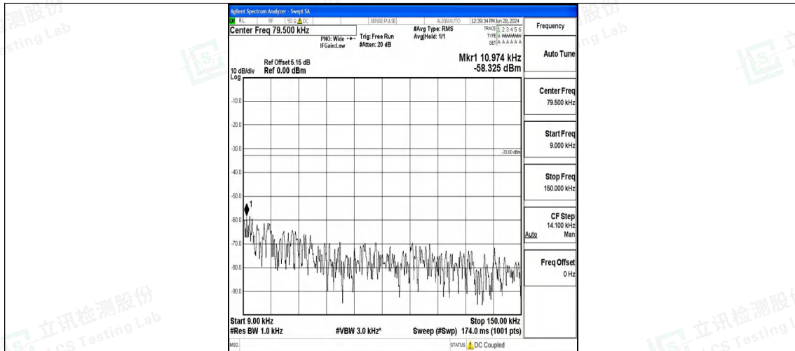
Band12_5MHz_QPSK_23155_1RB#0_0.009~0.15_0.009~0.15
