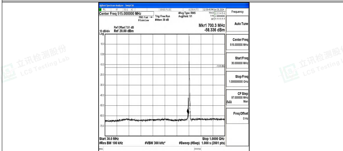
Band12_5MHz_QPSK_23155_1RB#0_30~1000_30~1000
