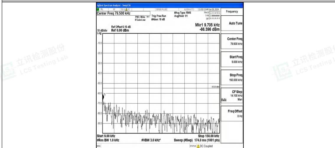
Band7_10MHz_16QAM_21400_1RB#0_0.009~0.15_0.009~0.15
