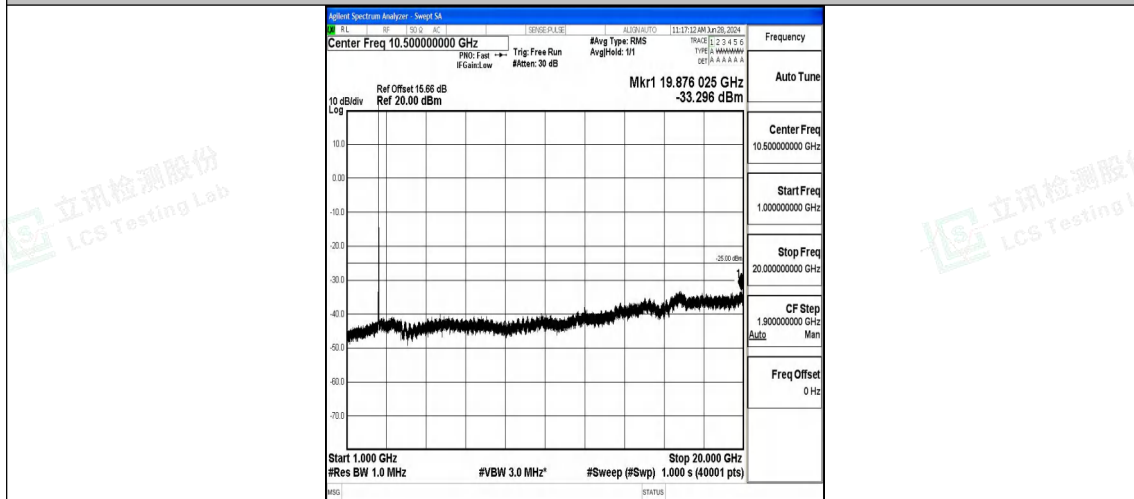
Band7_15MHz_QPSK_21100_1RB#0_1000~20000_1000~20000
