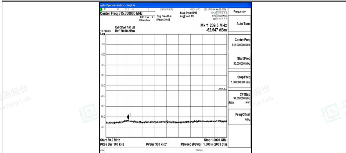
Band7_15MHz_QPSK_21100_1RB#0_30~1000_30~1000
