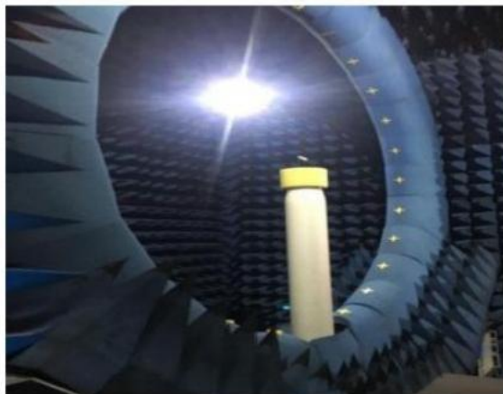
SATIMO Dark room
