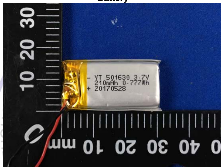
Battery
