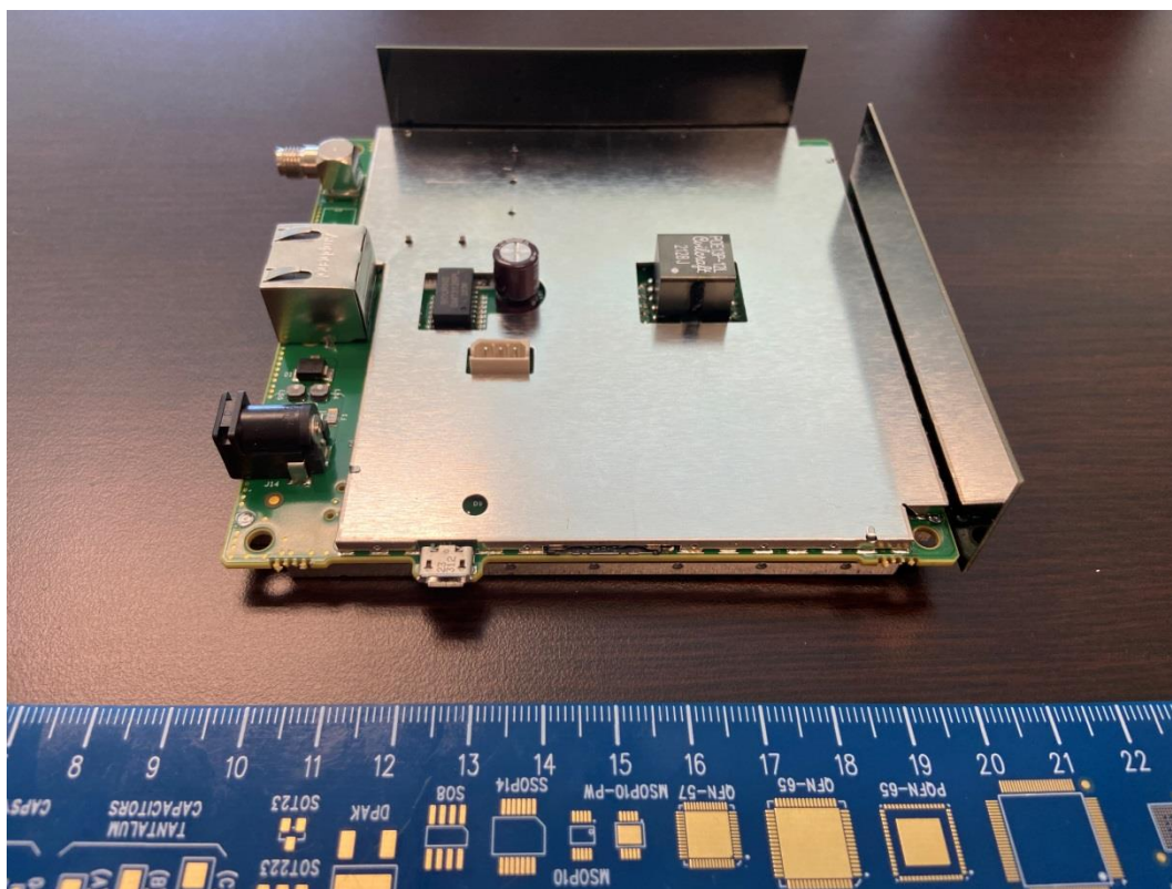
USB: PCB Bottom side
