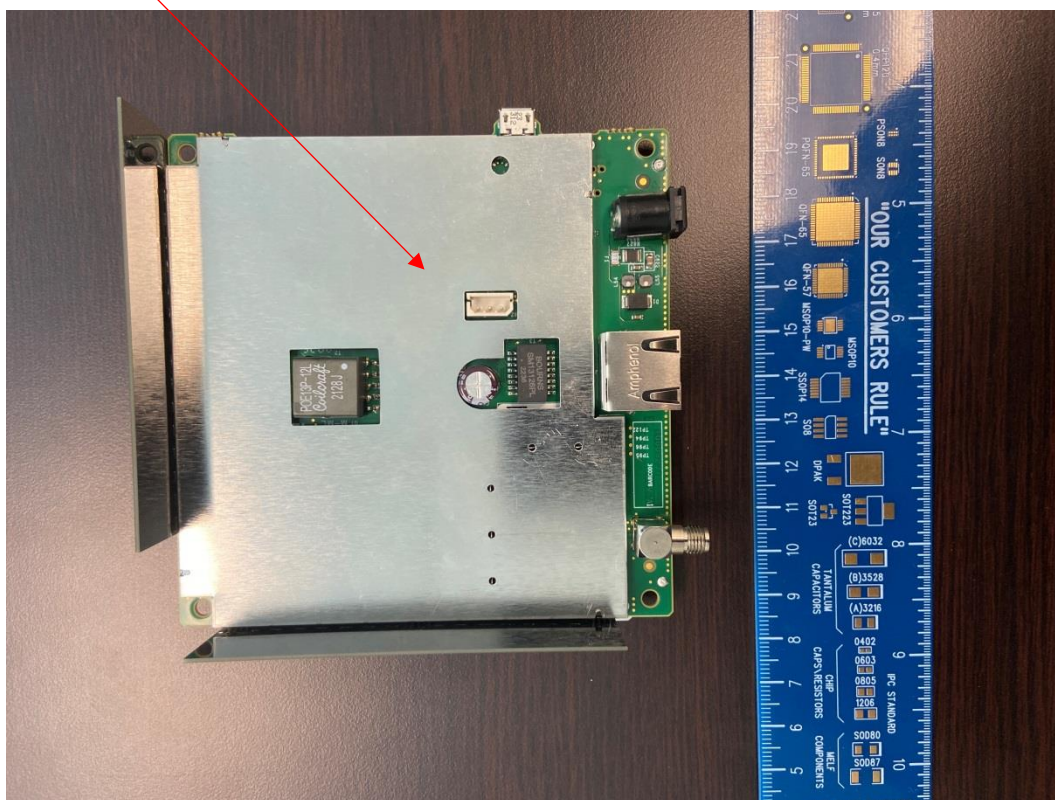
PCB Top View with Shield: PCB Bottom side
