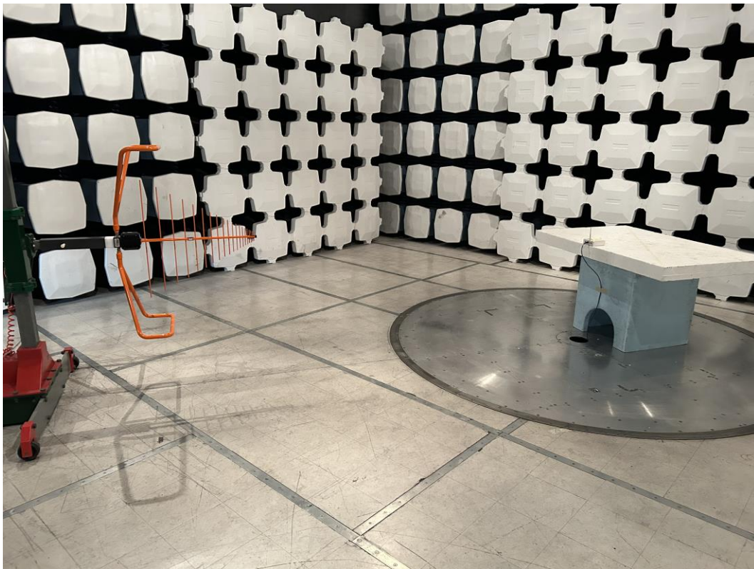
Radiated Emission 30 MHz to 1 GHz Test Setup:
