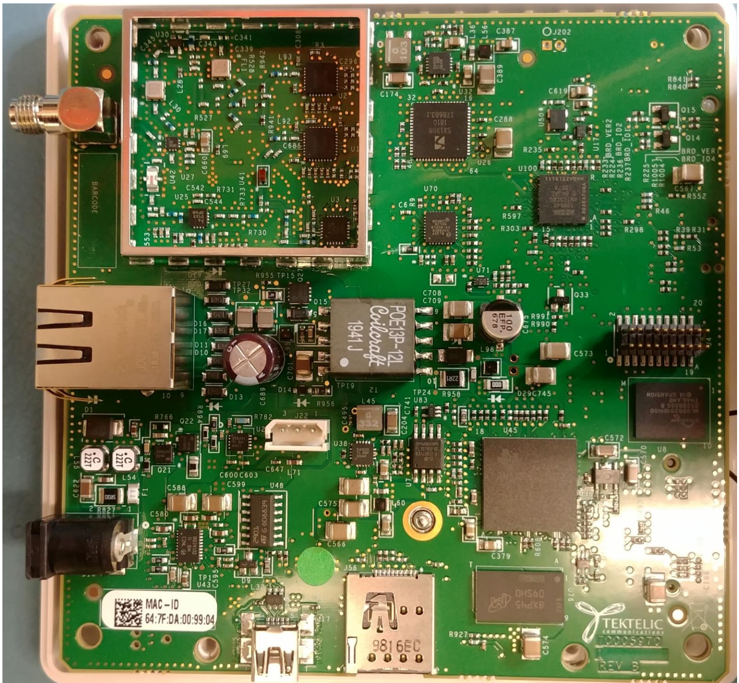
PCB unshielded Bottom View
