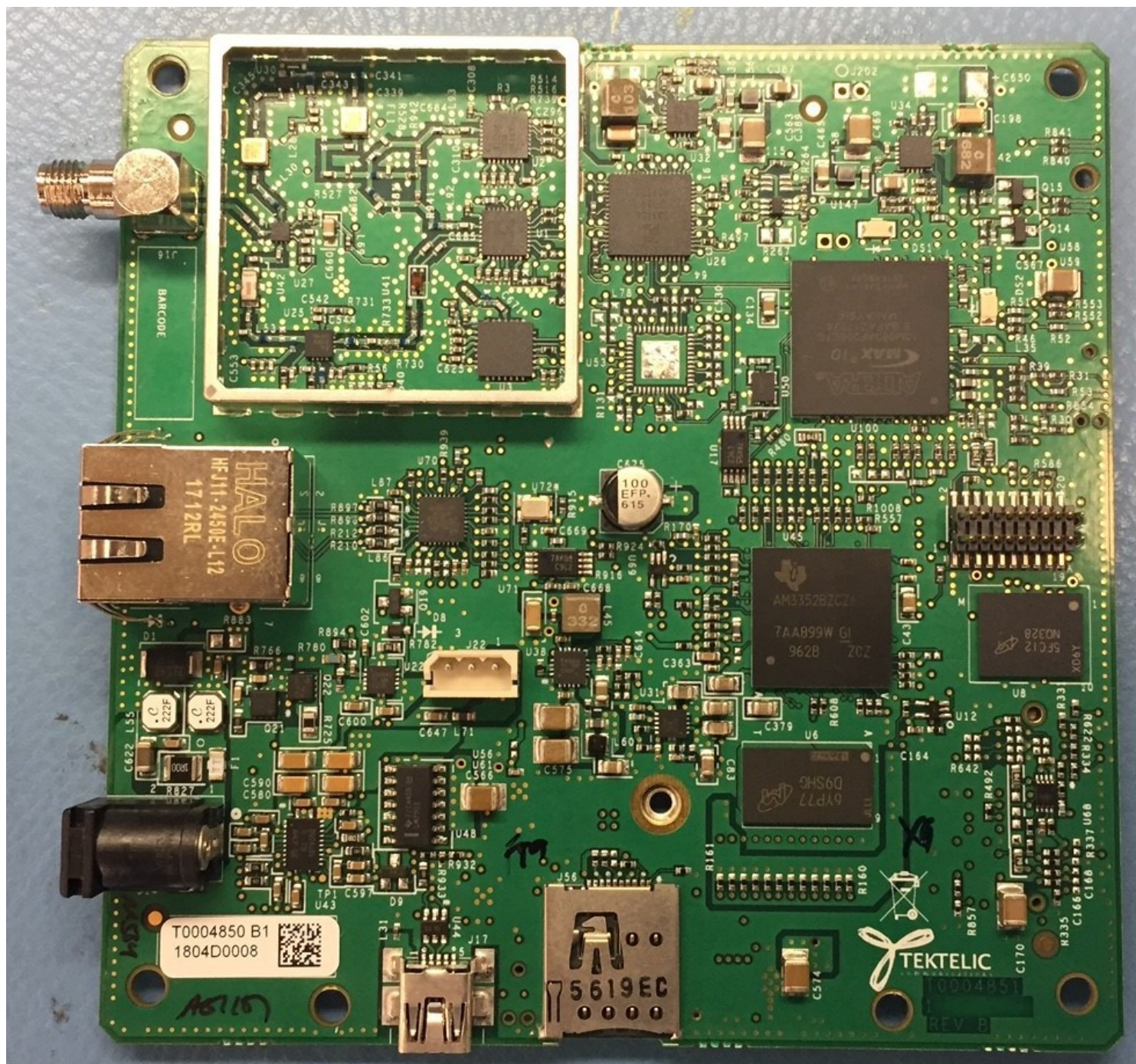
EUT: PCBA with LoRa Module (without Shield) Top view
