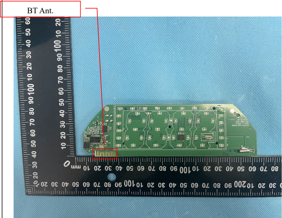
Antenna View 1
