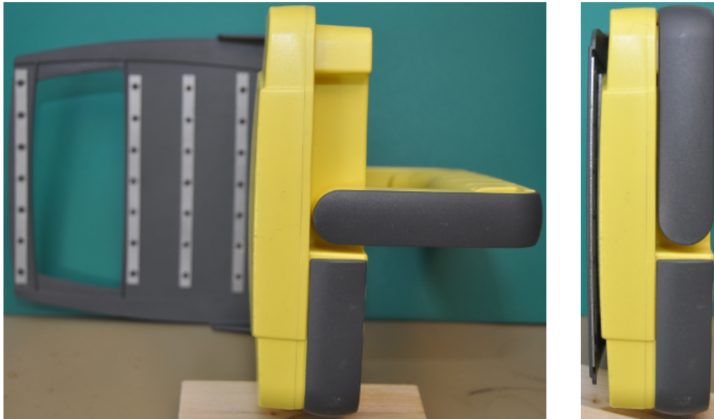
Figure 7: Recco detector bottom view, antenna and handle opened(left)/closed(right)
