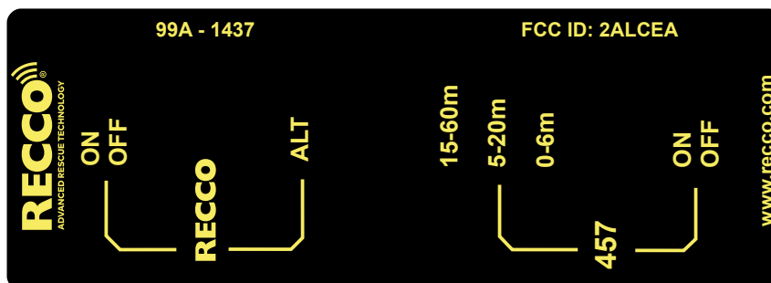
Figure 1: Recco detector Label (size 113x42mm)
