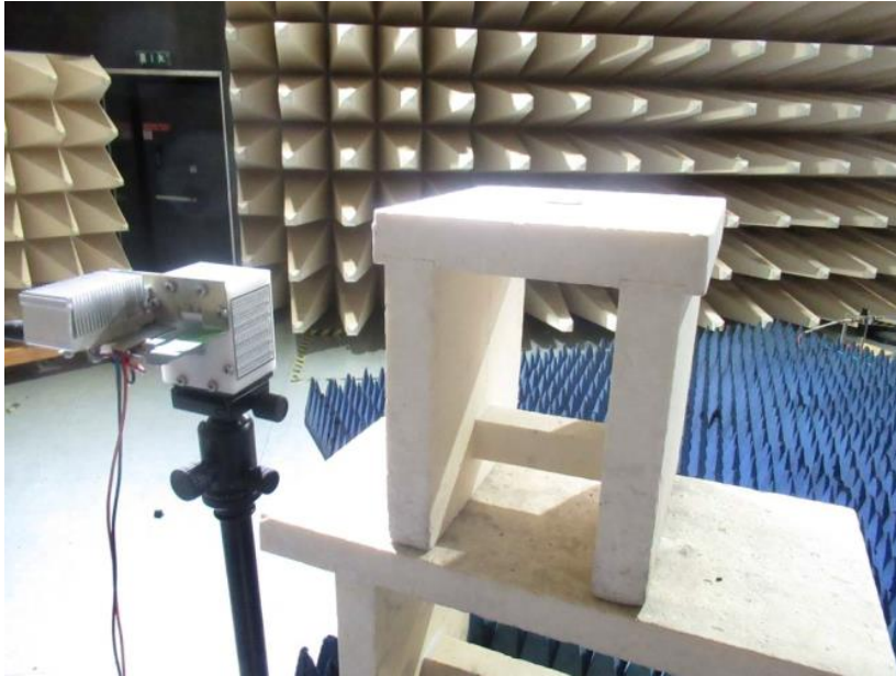
9. Radiated Emissions at 1164-1240 MHz and 1559-1610 MHz
