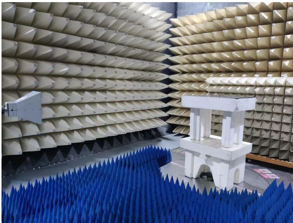
Photograph 2: Set-up photo for Radiated Emission, 1GHz - 5GHz
