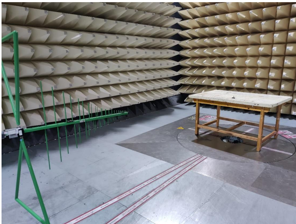
Photograph 1: Set-up photo for Radiated Emission, 30MHz - 1GHz
