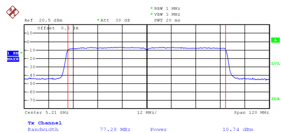
802.11ax(HT80) Low channel
