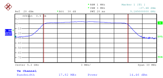
802.11n(HT20) middle channel
