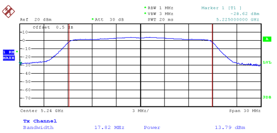
802.11n(HT20) high channel
