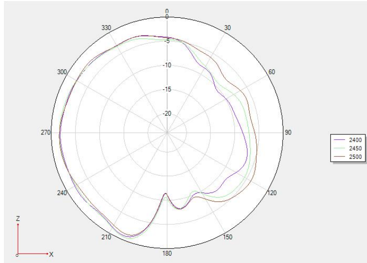
Phi 0 2Dfigure
