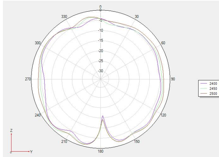
Phi 90 2Dfigure
