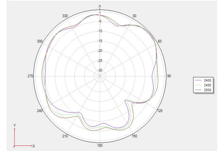
Theta 90 2Dfigure
