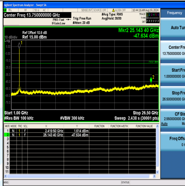
11AX40MIMO-Ant2-2422-1000~26500-PASS
