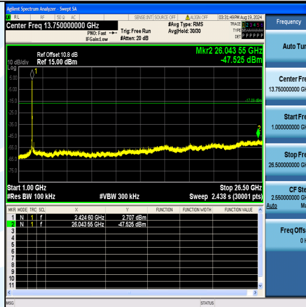
11AX40MIMO-Ant1-2437-0~Reference-PASS
