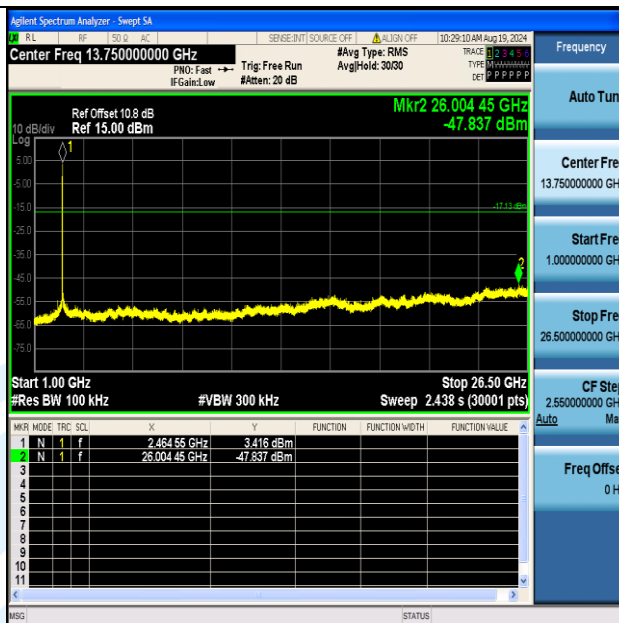
11AX20MIMO-Ant2-2462-1000~26500-PASS
